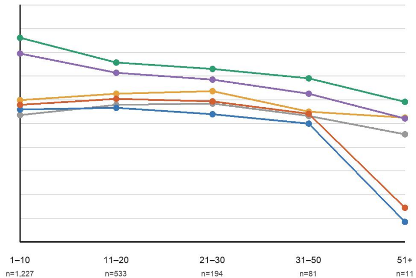
Qwen2.5-72B
