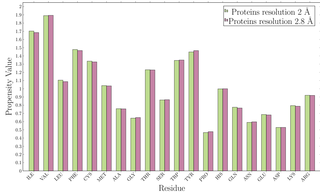
Amino Acid Propensity in Beta Strands
