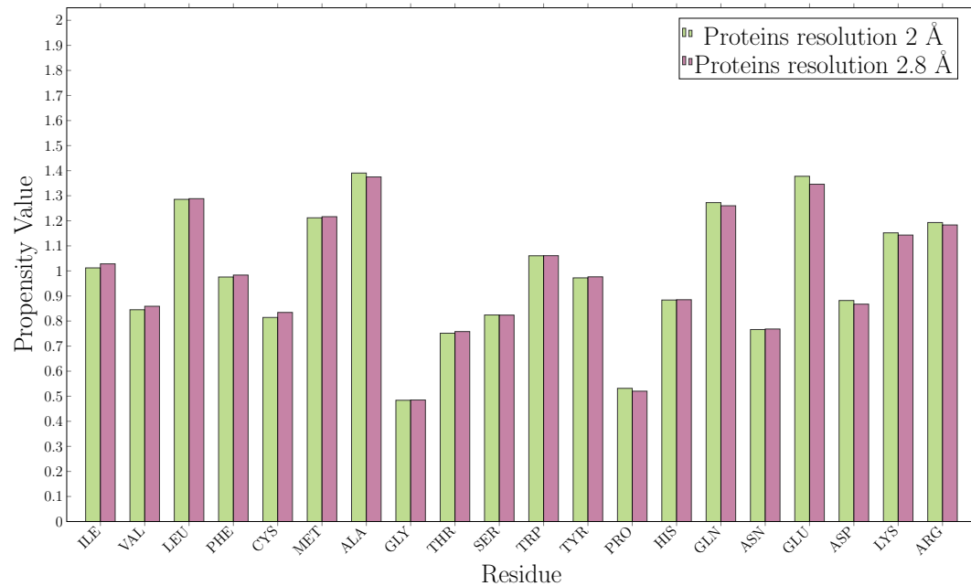
Amino Acid Propensity in Helices
