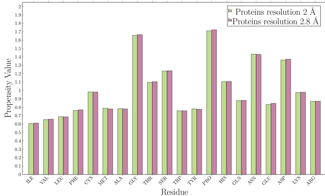
Amino Acid Propensity in Loops
