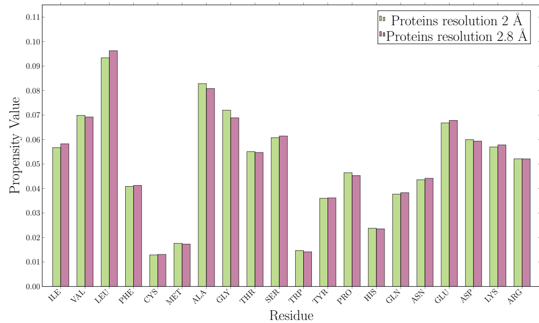
Amino Acid Probability in Proteins
