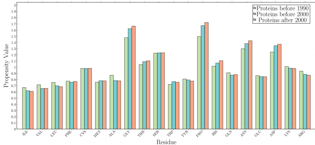
Amino Acid Propensity in Loops
