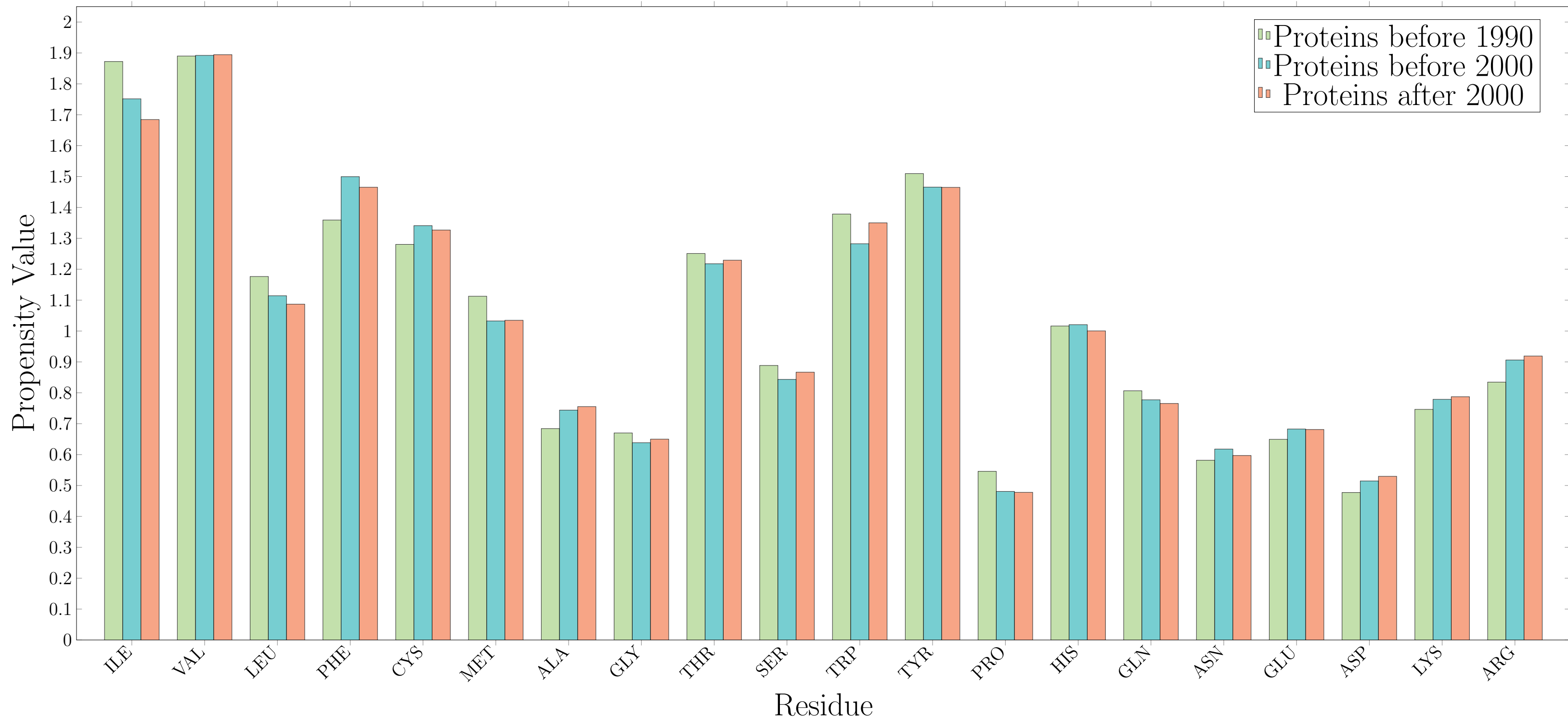
Amino Acid Propensity in Beta Strands
