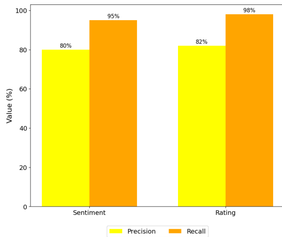
Fig. 2. Comparison of precision and recall between sentiment and rating.
