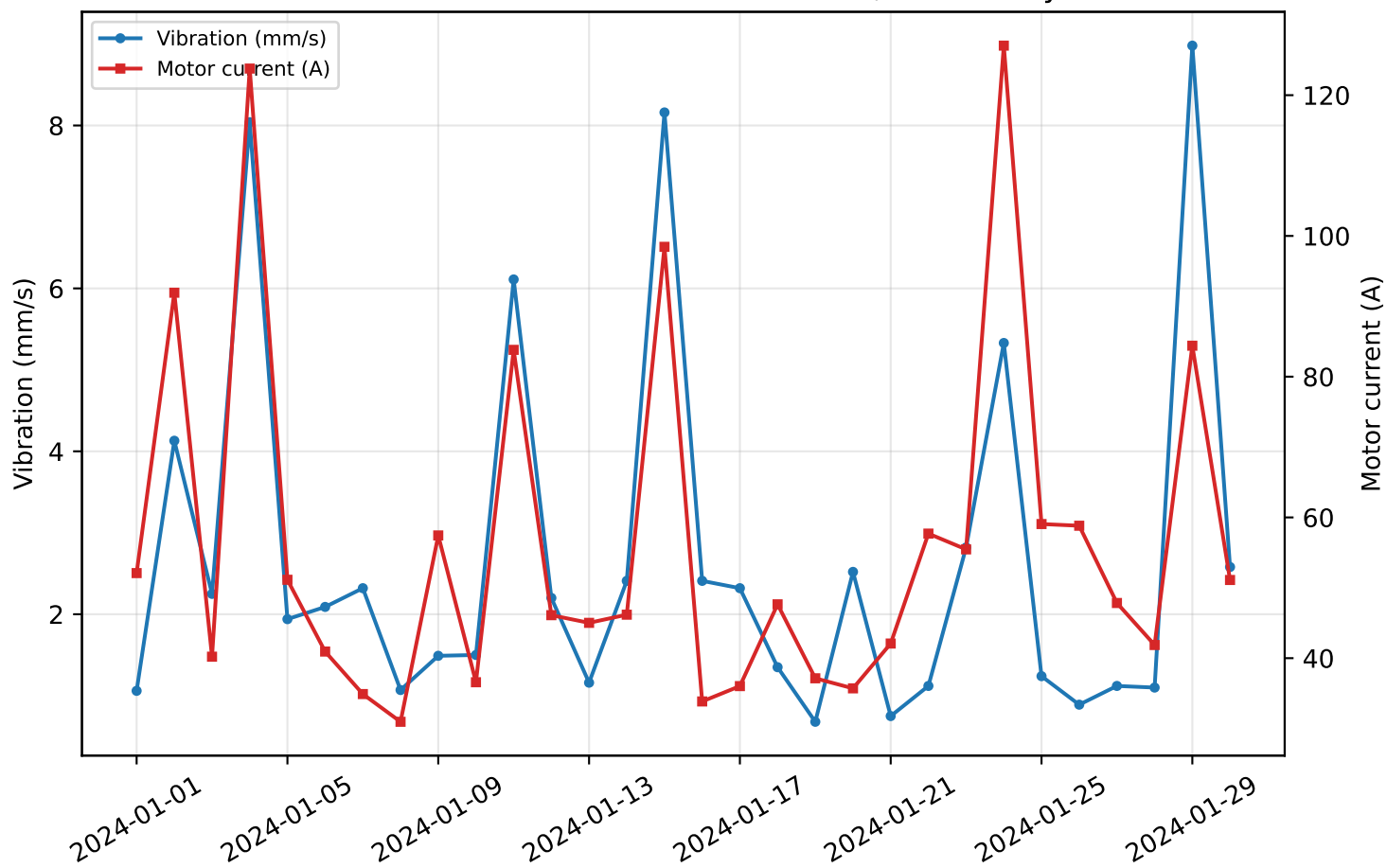
WELL-01 - vibration and motor current, last 30 days
