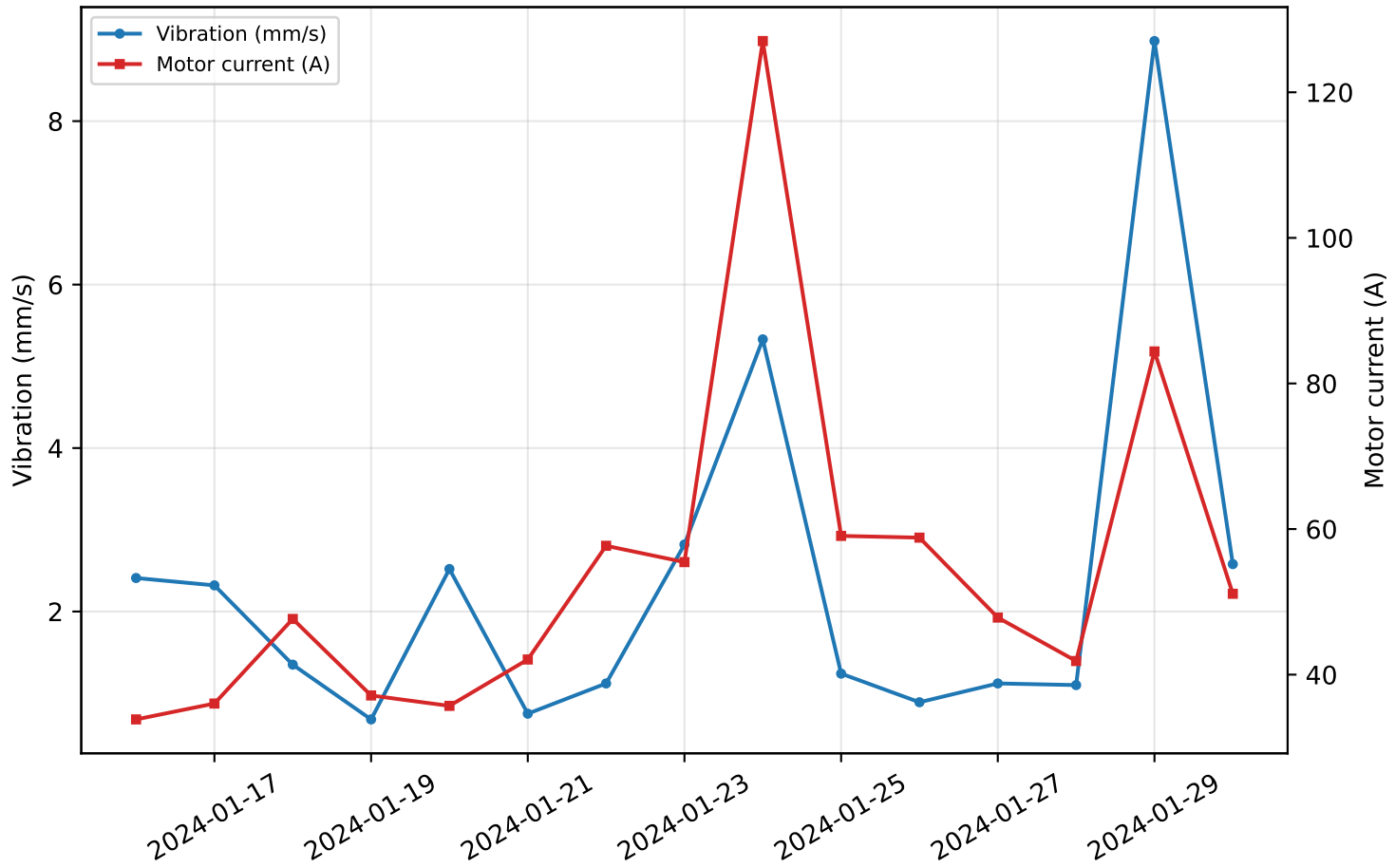
WELL-01 - vibration and motor current, last 15 days
