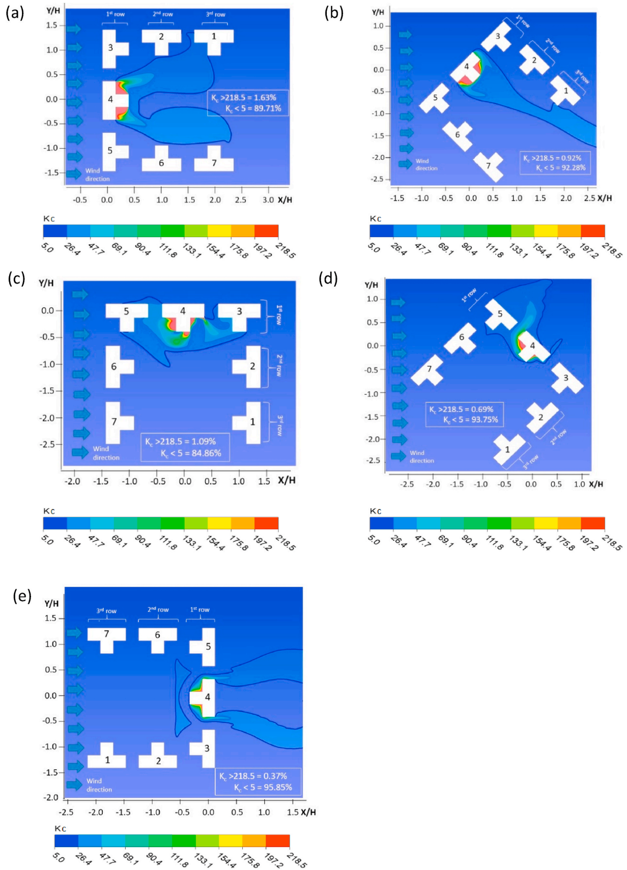
Fig. 13. Concentration distribution for 'U' arrangement with incident wind angles of: (a) 0^\circ , (b) 45^\circ , (c) 90^\circ , (d) 135^\circ , and (e) 180^\circ , at pedestrian height (8.75 mm in scaled model, 1.75 m in full scale).
