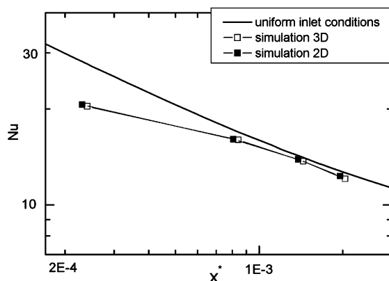
Fig. 9. Comparison of Nusselt number distributions along the channel between two and three-dimensional models. e = 1 mm, Re = 2166 , e^* = 12.4 .
