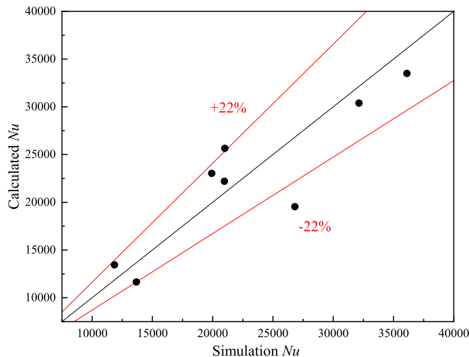
Fig. 23. The comparison of fitted values to simulated values when fitting the correlation using Re and Eu .
