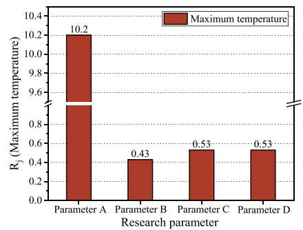
(a) Range analysis on maximum temperature
