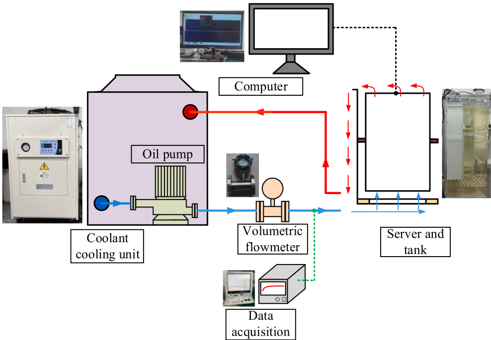
Fig. 9. Experiment system.
