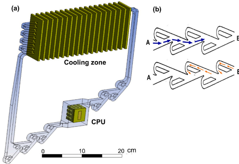
Fig. 2. (a) The design of the cooling system. The fluid domain is in blue, and CPU and radiator in the cooling zone are in brown. (b) A sketch of the asymmetric property of the Tesla valve. (For interpretation of the references to color in this figure legend, the reader is referred to the Web version of this article.)
