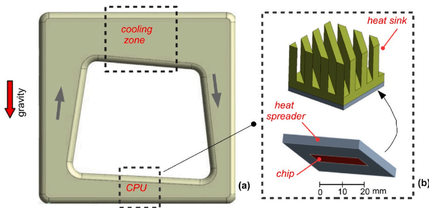
Fig. 1. (a) A sketch of a prototype of the recirculating cooling system with weak asymmetry in geometry. (b) Detail of the CPU component, which is used in the real design in Section 3.
