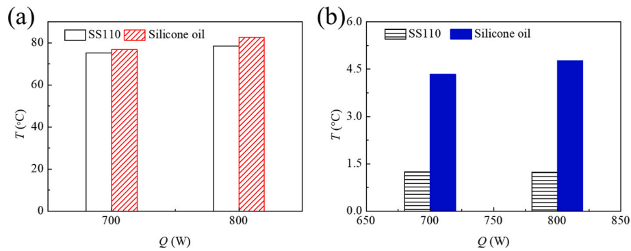
Fig. 29. Measured temperatures at identical locations under the same heating power and mass flow rate. (a) Average temperature; (b) Standard deviation of temperature.
