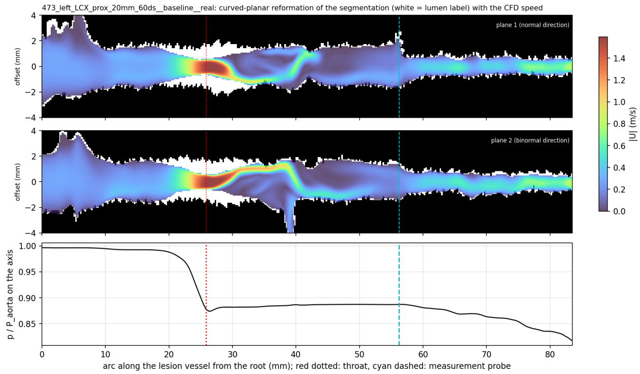
Figure 47: P5 scan 473 (LCx, 20 mm, 60%DS): same layout as for scan 138.
