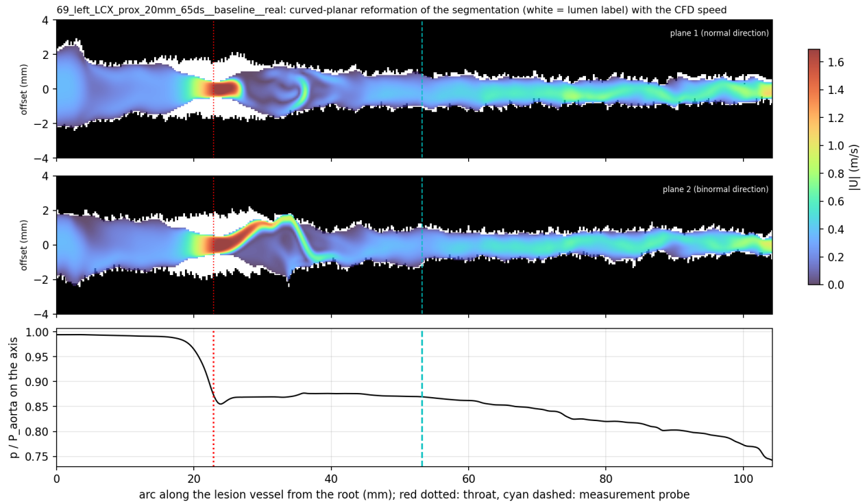
Figure 44: P5 scan 69 (LCx, 20 mm, 65%DS): same layout as for scan 138.
