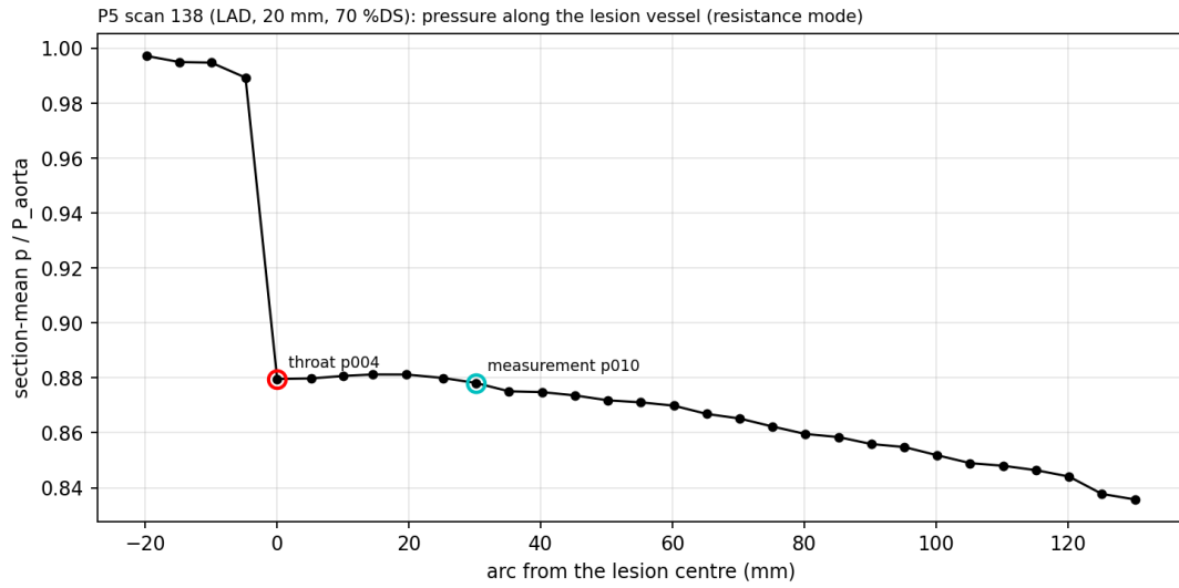
Figure 43: P5 scan 138: section-mean p/P_{aorta} at the package probes along the lesion vessel (resistance mode), with the throat and measurement probes marked.
