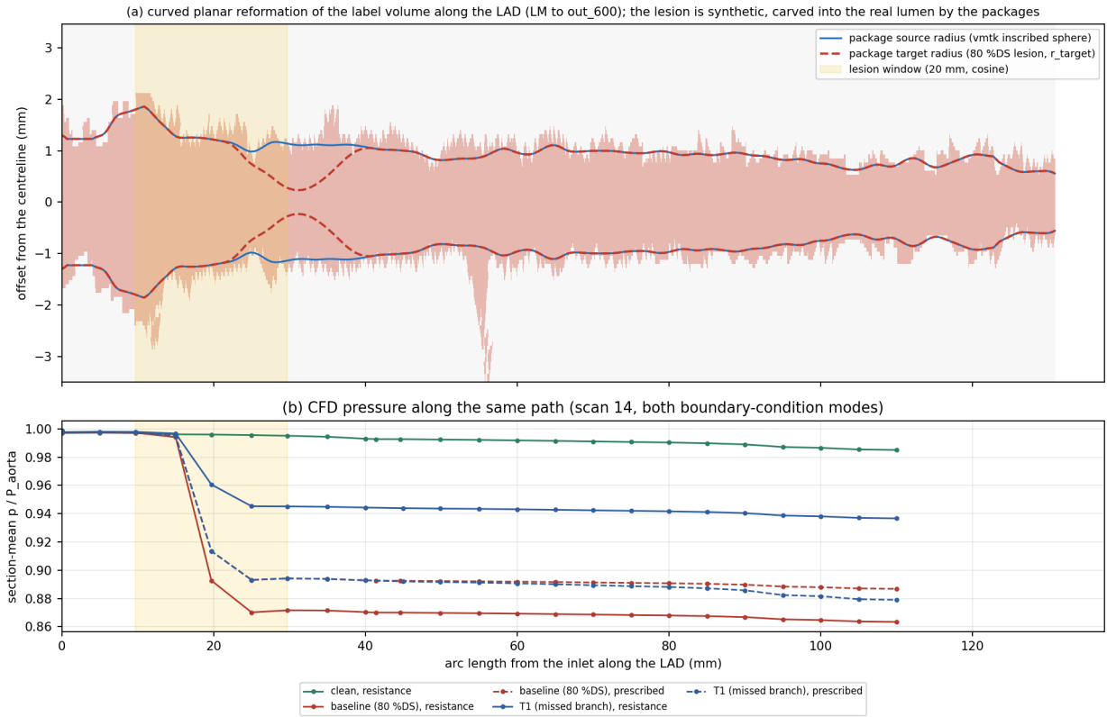
Figure 32: (a) Curved planar reformation of the scan-14 label volume along the LAD (LM to out_600) with the radii of the package: the source radius (blue) and the target radius of the 80%DS lesion (red dashed), which is synthetic and carved into the real lumen. (b) Section-mean pressure of the CFD solves along the same path in both boundary-condition modes.
