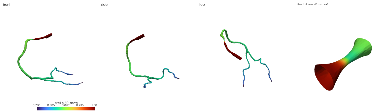
Figure 54: P5 scan 139: wall pressure p/P_{aorta} of the tree in three views and the 6 mm around the throat.
