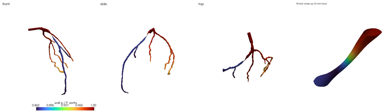
Figure 39: Variant A2 (zone interfaces shifted by 1 mm): wall pressure, same layout and colour scale as Fig. 38.
