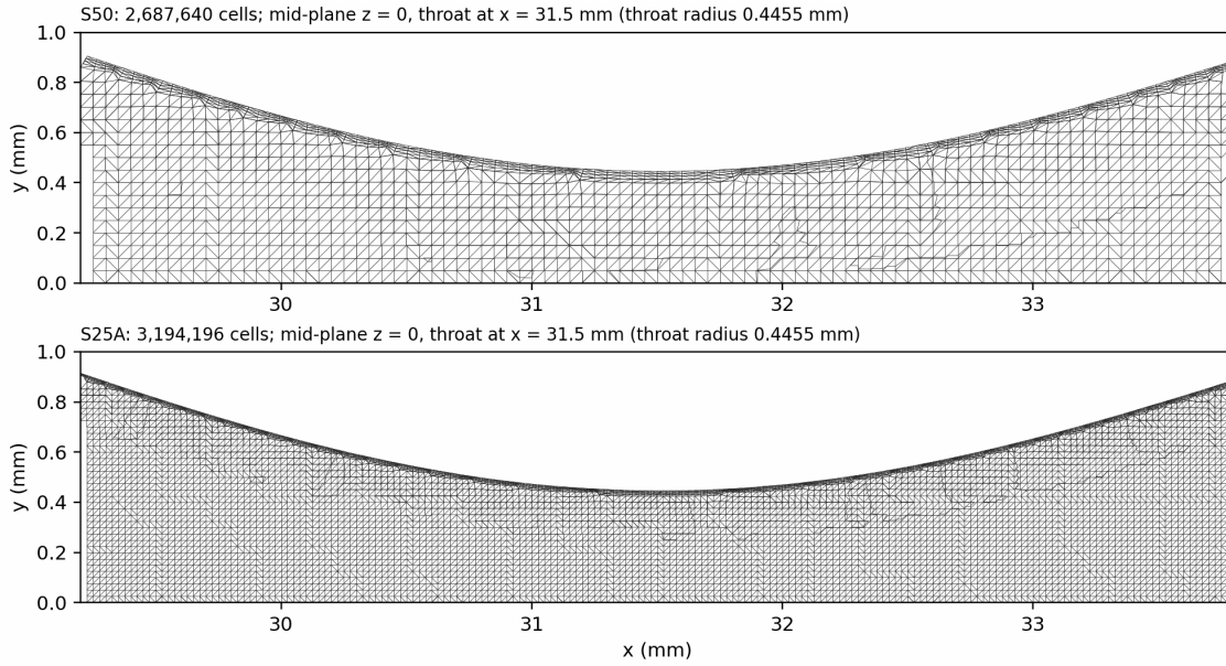
Figure 29: Throat-zone mesh of the U3D levels S50 ( 50\ \mu\text{m} ) and S25A ( 25\ \mu\text{m} ): cell edges in the mid-plane z = 0 , x = 29.2\text{--}33.8\text{ mm} , with the four-layer boundary stack along the wall. The meshes were rebuilt on 2026-10-02 from the deposited code (same cell counts as the returned levels; cartesianMesh is not bitwise reproducible, so individual cells may differ from the returned meshes). The diagonal lines are where the plane cuts the cells' faces, not extra cells. Script code_from_cfd/task1_u3d/jet_state_check/viz_u3d_meshes.py .
