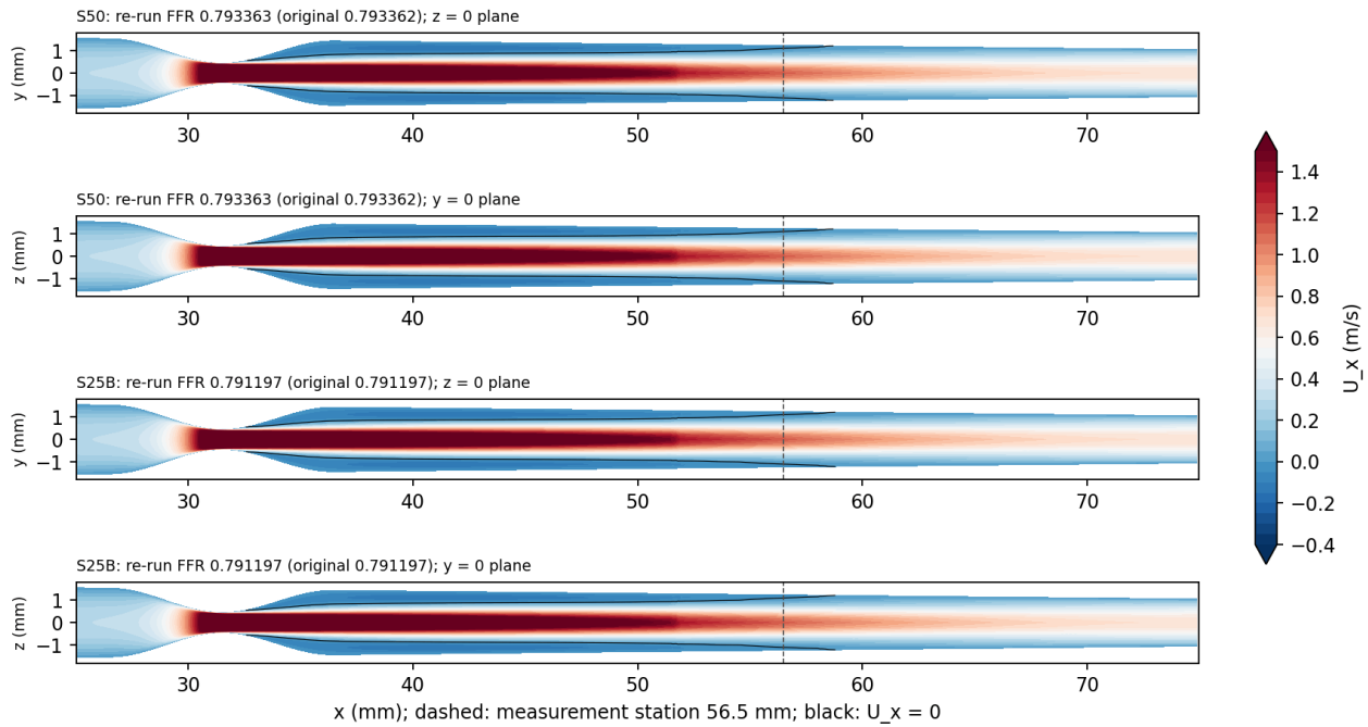
Figure 40: Task B: axial velocity on the two mid-planes of the re-run levels S50 and S25B (throat at 30 mm, U_x = 0 contour in black, dashed: measurement station 56.5 mm). Both jets are axisymmetric and the FFR equals the original value (to 10^{-6} and 3 \times 10^{-8} ). Script code_from_cfd/task_1003/viz/viz_u3d.states.py .
