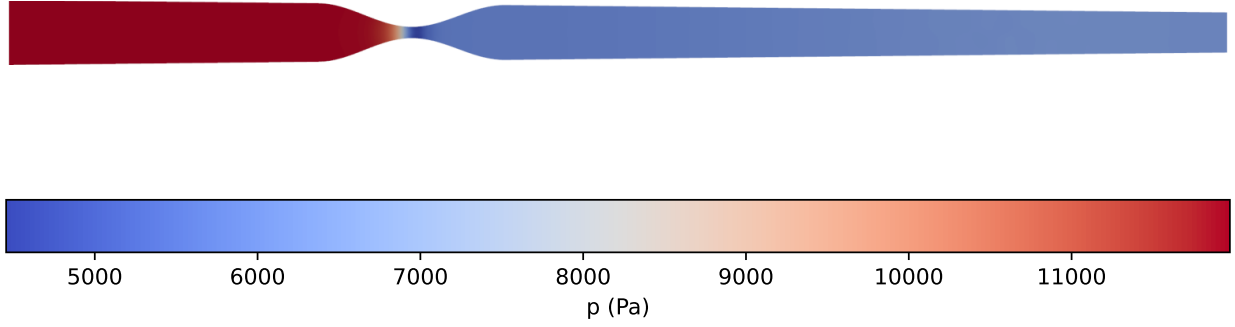
Figure 6: Pressure field over the same region and time state as the velocity figure above, showing the expected smooth pressure drop through the stenosis.
