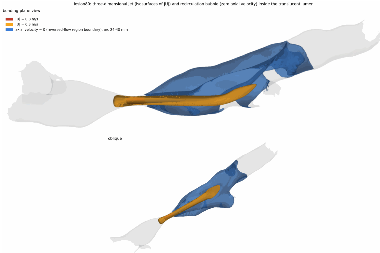
Figure 19: Lesion80, three-dimensional structure of the flow: isosurfaces of |U| = 0.3 m/s (orange) and 0.8 m/s (red) show the jet leaving the throat as a slender core that bends towards the wall; the blue surface is the zero-axial-velocity surface for arc 24–40 mm and encloses the recirculation region, which wraps around the jet (it touches the wall over much of its extent). Two views; translucent grey: lumen.
