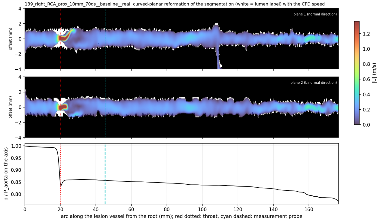
Figure 53: P5 scan 139 (RCA, 10 mm, 70%DS): same layout as for scan 138.
