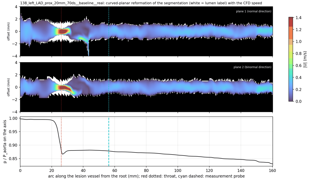
Figure 41: P5 scan 138 (LAD, 20 mm, 70%DS): curved-planar reformation of the unmodified lumen label (white) in two orthogonal planes with the CFD speed |U| in the CFD domain (the synthetic stenosis exists only in the CFD surface), and p/P_{aorta} on the axis (bottom); red dotted: throat, cyan dashed: measurement probe.
