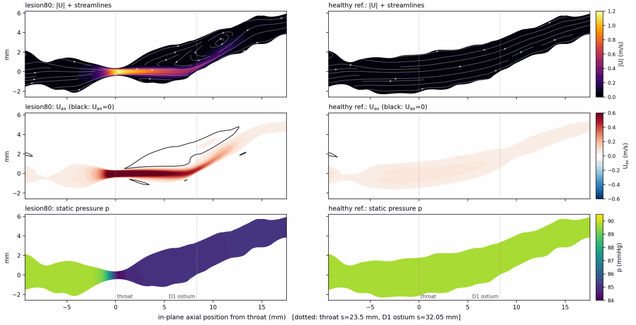
Figure 15: Longitudinal section through the LAD in its bending plane, lesion80 (left) and healthy reference (right), arc \approx 14\text{--}41 mm: |U| with in-plane streamlines, axial velocity with the zero contour, static pressure. The jet from the 0.75 mm throat stays narrow for about 5 mm and is then deflected along one wall; on the other side the zero-velocity contour encloses a recirculation region beginning about 1 mm downstream of the throat and reaching past the D1 ostium (dotted), with a closed vortex visible in the streamlines about 10–12 mm downstream; a second, small reversed pocket lies on the opposite wall 1–3.5 mm downstream. The healthy vessel shows uniform low-speed forward flow. Colour scales are identical in both columns.
