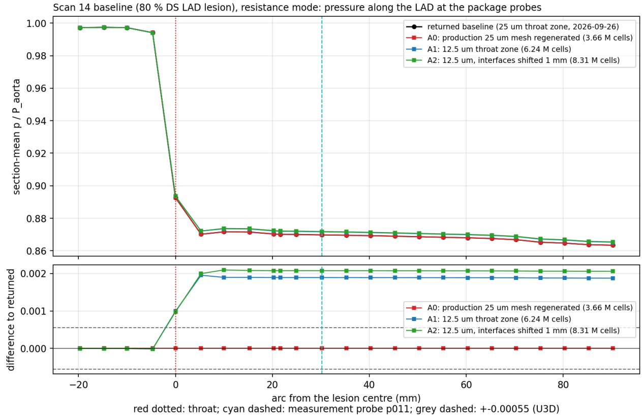
Figure 35: Task A: section-mean p/P_{aorta} at the package probes along the LAD for the returned baseline (25 \mu m), the control A0 (regenerated 25 \mu m), A1 and A2 (12.5 \mu m), and the differences (lower panel; dashed: \pm U_{3D} ). A0 coincides with the returned baseline; A1 and A2 are identical upstream of the lesion and offset by about +0.002 downstream.
