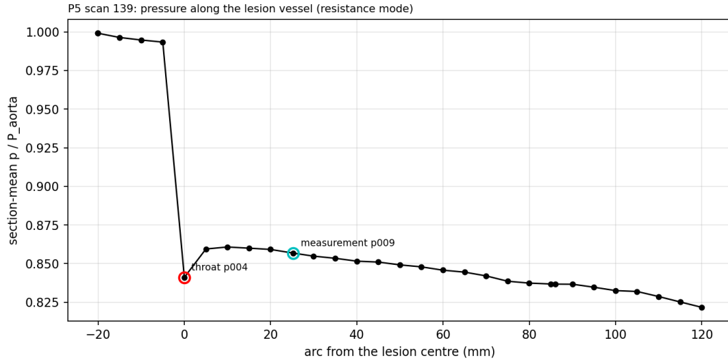
Figure 55: P5 scan 139: section-mean p/P_{aorta} along the lesion vessel at the package probes.
