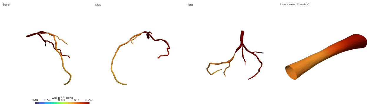
Figure 42: P5 scan 138: wall pressure p/P_{aorta} of the tree in three views and the 6 mm around the throat.
