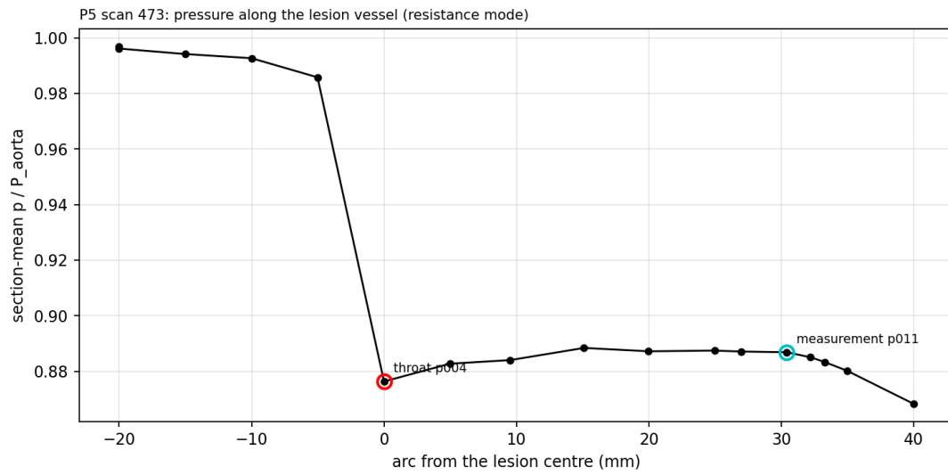
Figure 49: P5 scan 473: section-mean p/P_{aorta} along the lesion vessel at the package probes.
