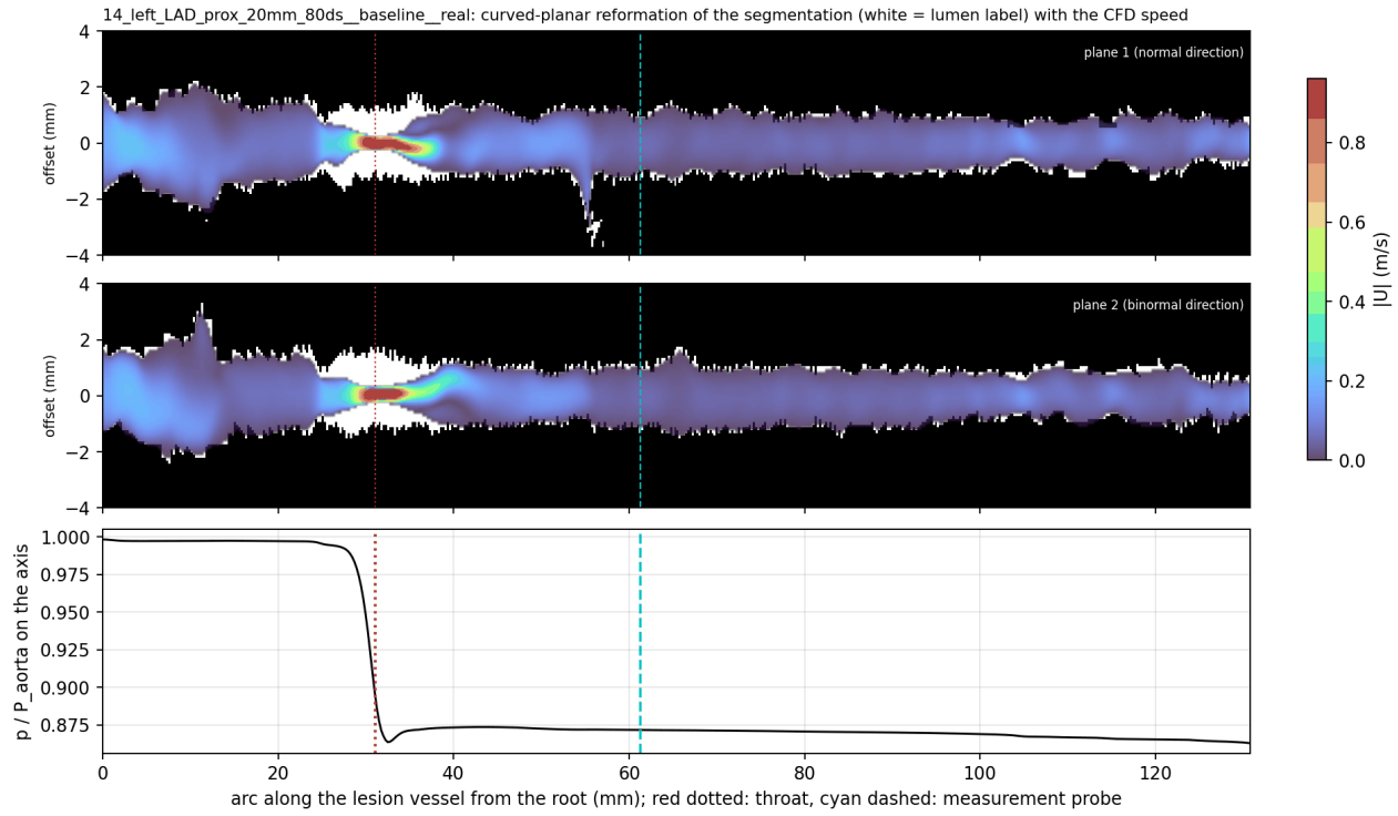
Figure 36: Imaging part, variant A1: curved-planar reformation of the unmodified ImageCAS-X lumen label (white) along the lesion vessel in two orthogonal planes with the CFD speed |U| in the CFD domain, and p/P_{aorta} on the axis (bottom). The synthetic 80% stenosis exists only in the CFD surface: the label is wider than the CFD lumen at the throat (white margins). Red dotted: throat; cyan dashed: measurement probe p011. Script code from_cfd/task_1003/viz/viz.imaging.py .
