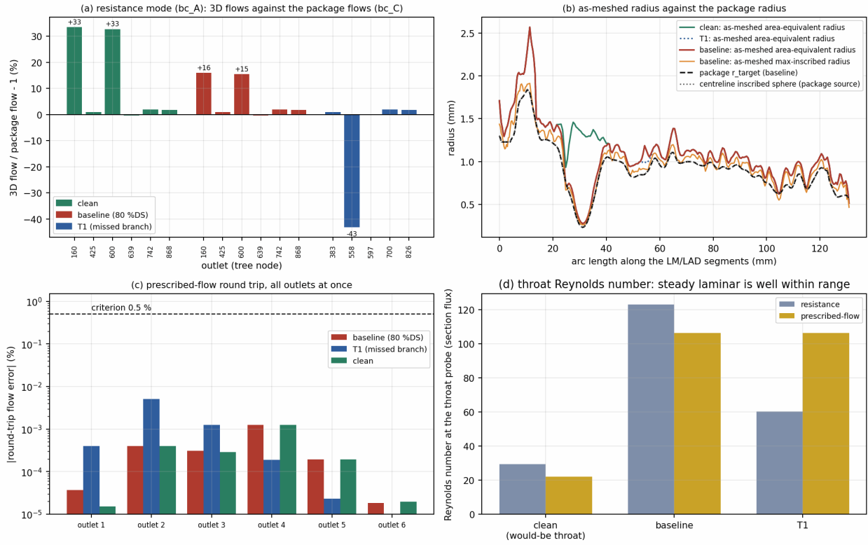
Figure 33: Scan 14, Gate M1: (a) resistance mode, 3D outlet flows against the package flows (bc_C); (b) as-meshed area-equivalent and maximum-inscribed radius along the LM/LAD segments against the package radius; (c) round-trip flow errors of the prescribed-flow mode (all outlets at once); (d) throat Reynolds number from the section flux.
