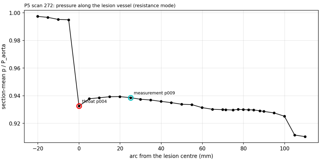
Figure 52: P5 scan 272: section-mean p/P_{aorta} along the lesion vessel at the package probes.
