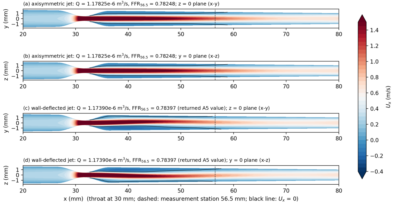
Figure 34: The two steady states of the Stage A sten70 case on the same mesh (the smoke-test mesh of 2026-10-01; state (c,d) obtained by restarting from the archived deflected solution): axial velocity on the two mid-planes, with the U_x = 0 contour (black). (a,b) axisymmetric jet; (c,d) jet deflected towards +y , -z , the state of the returned A5 coarse value. Both are converged (flow band below 10^{-4}\% over 4000 iterations). Script code_from_cfd/task_0926/fig_two_states.py ; jet-offset diagnostic jet_offset.py .
