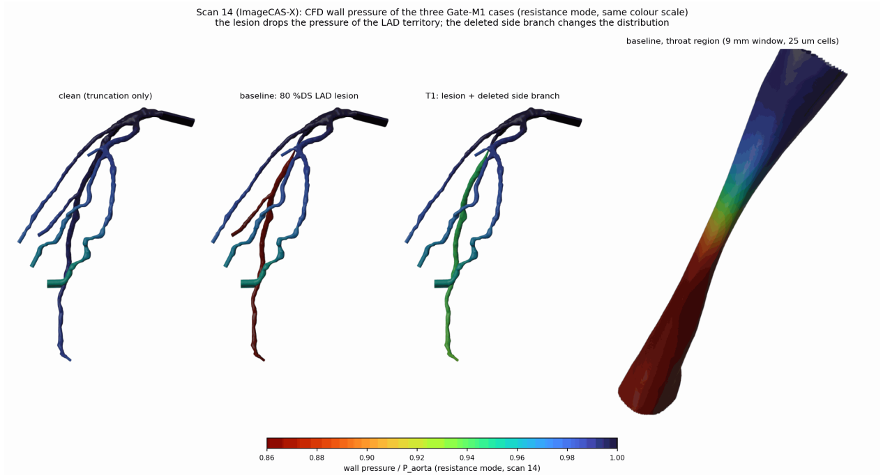
Figure 31: Scan 14, wall pressure over aortic pressure of the three cases in resistance mode (same colour scale; Blender, Workbench engine). The 80%DS lesion drops the pressure of the LAD territory to 0.86–0.87 of the aortic pressure; in T1 the deleted side branch changes the distribution (out_558, whose full-territory target cannot be delivered, is depressed). Right: the throat region of the baseline mesh.
