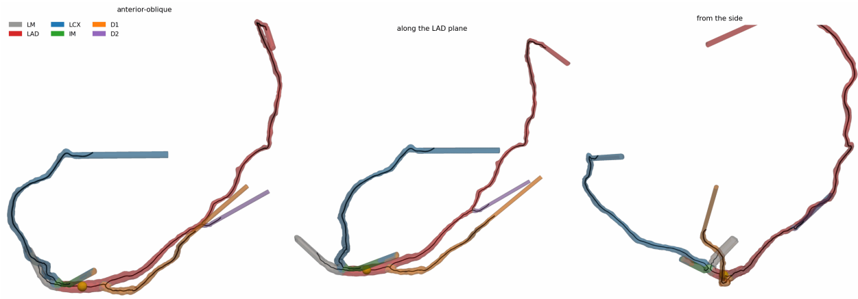
Figure 11: Left coronary tree of scan 837 as used for the CFD: the rebuilt segmentation surface (clipped at the 0D truncation, 20 mm straight outlet extensions, translucent), coloured by 0D-tree branch (LM grey, LAD red, LCX blue, IM green, D1 orange, D2 purple), the extracted centreline inside the lumen (black), and the lesion80 throat (yellow sphere, LAD arc 23.5 mm). Three views.
