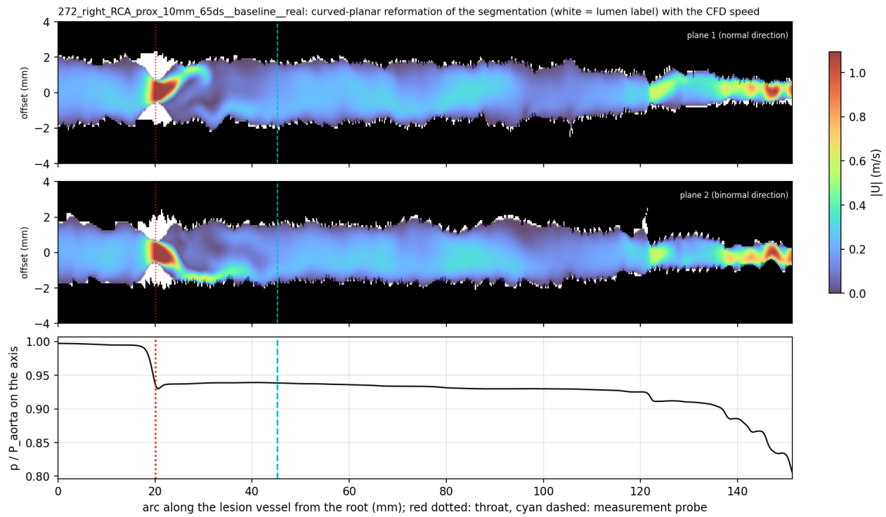
Figure 50: P5 scan 272 (RCA, 10 mm, 65%DS; the outlet out_396 was lost in the mesh and is absent from the solve): same layout as for scan 138.
