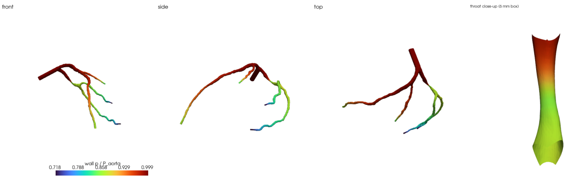
Figure 45: P5 scan 69: wall pressure p/P_{aorta} of the tree in three views and the 6 mm around the throat.
