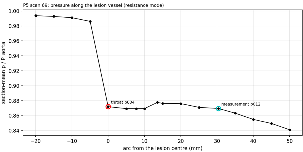
Figure 46: P5 scan 69: section-mean p/P_{aorta} along the lesion vessel at the package probes.
