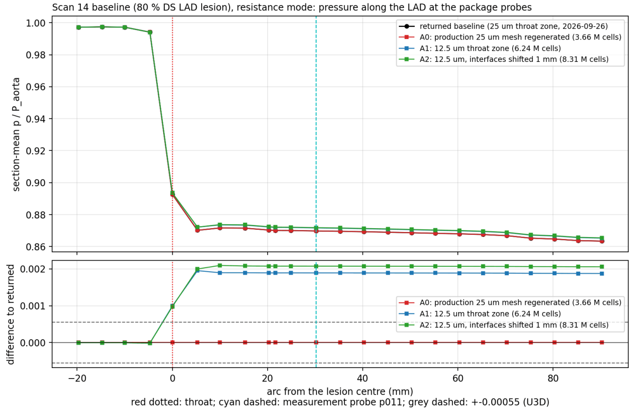
Figure 35: Task A: section-mean p/P_{\text{aorta}} at the package probes along the LAD for the returned baseline (25 \mu\text{m} ), the control A0 (regenerated 25 \mu\text{m} ), A1 and A2 (12.5 \mu\text{m} ), and the differences (lower panel; dashed: \pm U_{3D} ). A0 coincides with the returned baseline; A1 and A2 are identical upstream of the lesion and offset by about +0.002 downstream.
