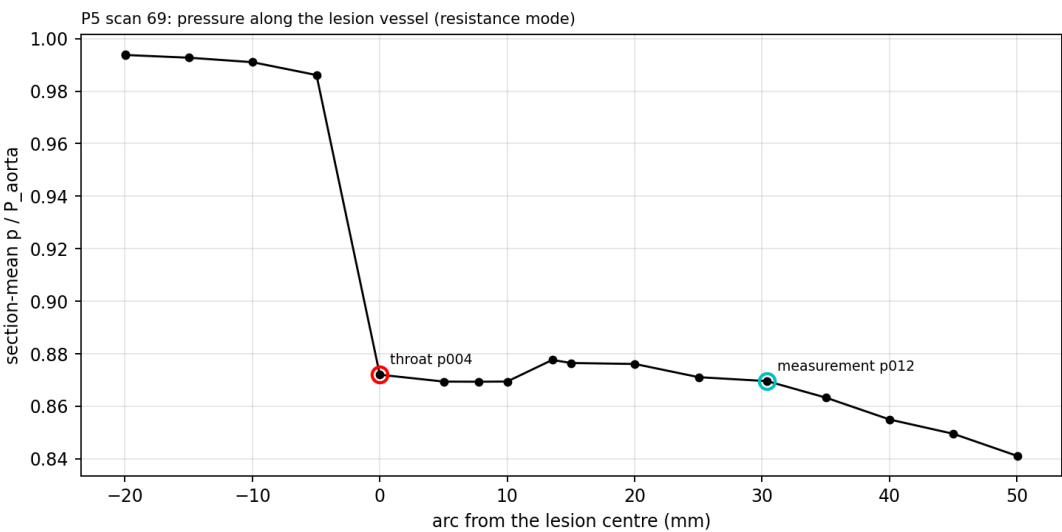
Figure 46: P5 scan 69: section-mean p/P_{\text{aorta}} along the lesion vessel at the package probes.
