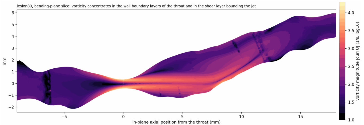
Figure 20: Vorticity magnitude |\nabla \times \mathbf{U}| on the bending-plane slice of lesion80 ( \log_{10}, 1/\text{s} ): the throat wall boundary layers ( \gtrsim 10^4 1/\text{s} ) and the thin shear layer bounding the jet stand out against the low-vorticity recirculation. The thin dark streaks crossing the vessel (at about -6.5 , 3\text{--}4 and 9\text{--}12 \text{ mm} ) are artefacts of the velocity-gradient computation across mesh-refinement interfaces, not flow features.
