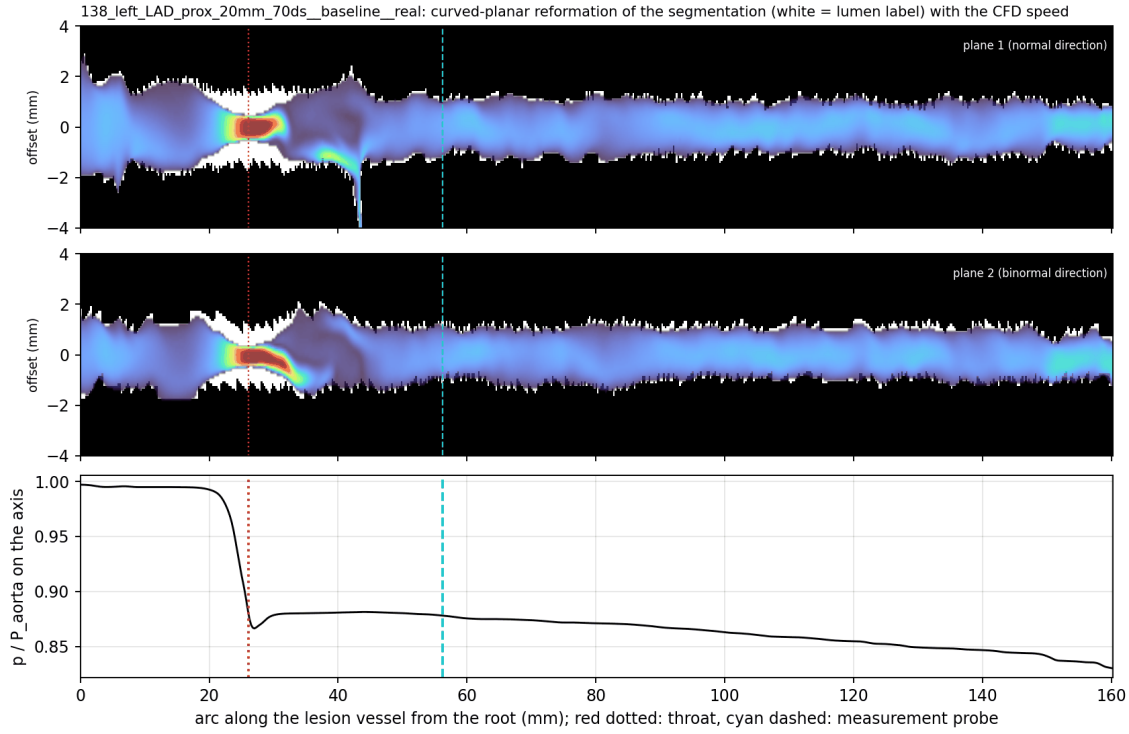
Figure 40: P5 scan 138 (LAD, 20 mm, 70%DS): curved-planar reformation of the unmodified lumen label (white) in two orthogonal planes with the CFD speed |U| in the CFD domain (the synthetic stenosis exists only in the CFD surface), and p/P_{aorta} on the axis (bottom); red dotted: throat, cyan dashed: measurement probe.
