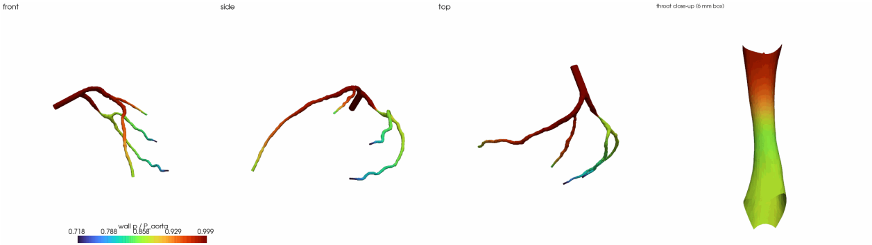
Figure 45: P5 scan 69: wall pressure p/P_{aorta} of the tree in three views and the 6 mm around the throat.
