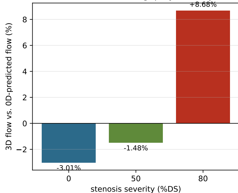
A2: 3D-vs-0D flow gap by severity
