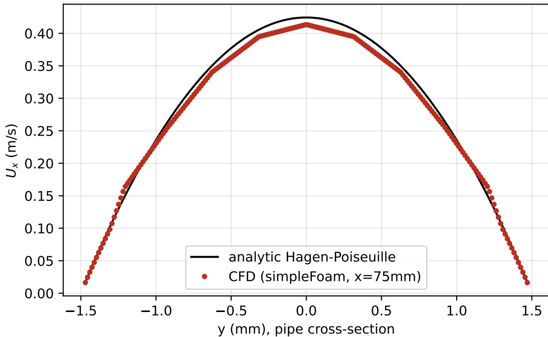
A1: Poiseuille pipe velocity profile CFD vs. analytic (fully-developed region)
