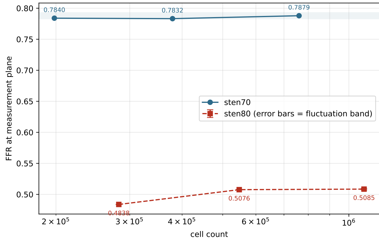
A5: mesh-independence study (shaded band: \pm 0.005 tolerance around sten70's finest level)
