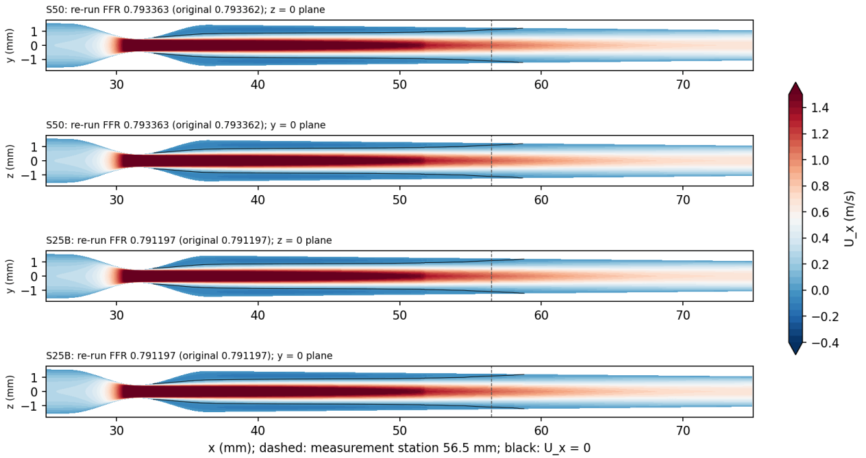
Figure 38: Task B: axial velocity on the two mid-planes of the re-run levels S50 and S25B (throat at 30 mm, U_x = 0 contour in black, dashed: measurement station 56.5 mm). Both jets are axisymmetric and the FFR equals the original value (to 10^{-6} and 3 \times 10^{-8} ). Script code_from.cfd/task_1003/viz/viz_u3d_states.py .
