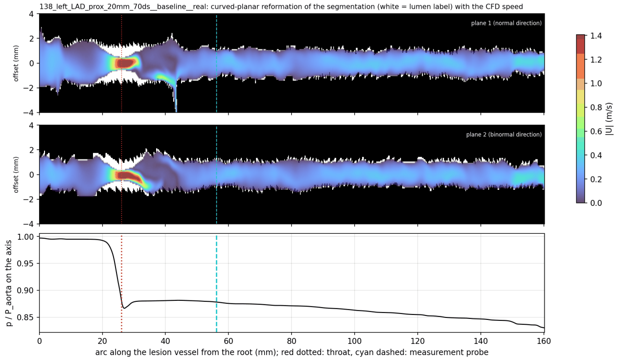
Figure 39: P5 scan 138 (LAD, 20 mm, 70%DS): curved-planar reformation of the unmodified lumen label (white) in two orthogonal planes with the CFD speed |U| in the CFD domain (the synthetic stenosis exists only in the CFD surface), and p/P_{\text{aorta}} on the axis (bottom); red dotted: throat, cyan dashed: measurement probe.
