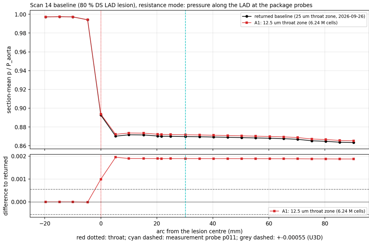
Figure 35: Task A, variant A1 (throat zone 12.5\ \mu\text{m} ): section-mean p/P_{\text{aorta}} at the package probes along the LAD against the returned baseline ( 25\ \mu\text{m} ), and the difference (lower panel; dashed: \pm U_{3D} ). Identical upstream of the lesion, a constant offset of +0.0019 downstream.
