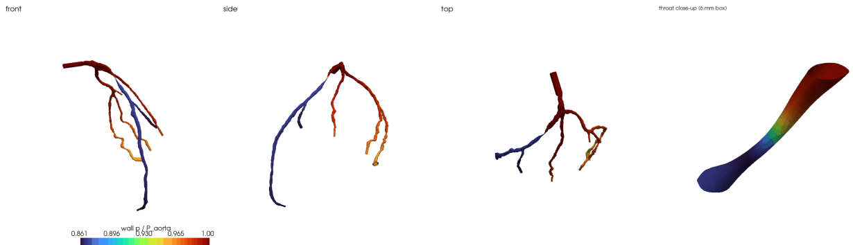
Figure 37: Variant A1: wall pressure p/P_{aorta} of the whole left coronary tree in three views and a close-up of the 6 mm around the throat (same colour scale).
