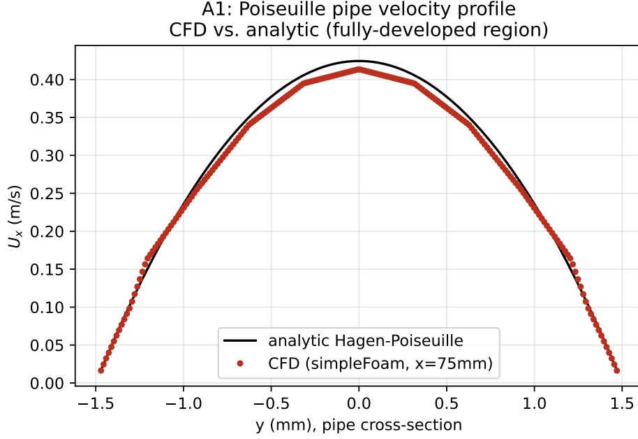
Figure 1: A1: velocity profile at x = 75 mm (fully-developed region) against the analytic Hagen–Poiseuille parabola. Peak-velocity agreement is -2.66\% , slightly larger than the -0.75\% pressure-drop error since a point value (peak velocity) is more sensitive to local profile shape than an integral quantity (pressure drop) is.
