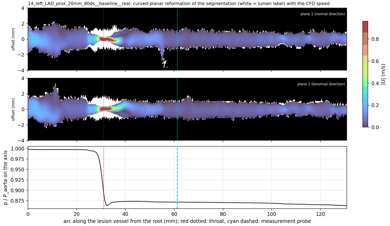
Figure 36: Imaging part: curved-planar reformation of the unmodified ImageCAS-X lumen label (white) along the lesion vessel in two orthogonal planes with the CFD speed |U| of variant A1 in the CFD domain, and p/P_{aorta} on the axis (bottom). The synthetic 80% stenosis exists only in the CFD surface: the label is wider than the CFD lumen at the throat (white margins), and the jet leaves the throat towards the distal vessel. Red dotted: throat; cyan dashed: measurement probe p011. Script code from_cfd/task.1003/viz/viz_imaging.py .
