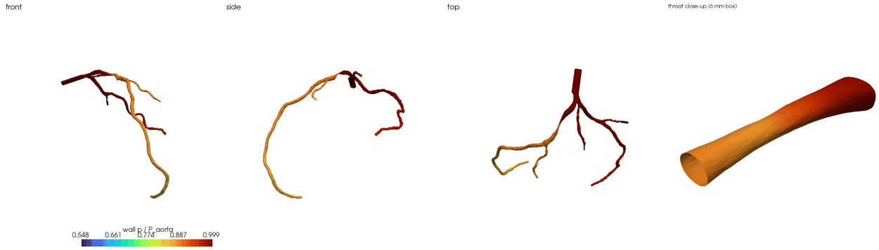
Figure 40: P5 scan 138: wall pressure p/P_{aorta} of the tree in three views and the 6 mm around the throat.
