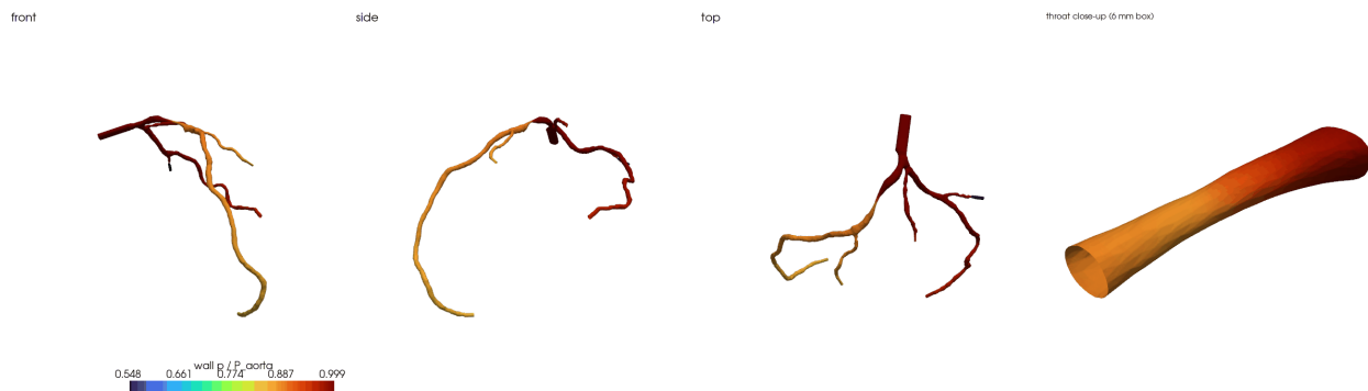
Figure 42: P5 scan 138: wall pressure p/P_{\text{aorta}} of the tree in three views and the 6 mm around the throat.
