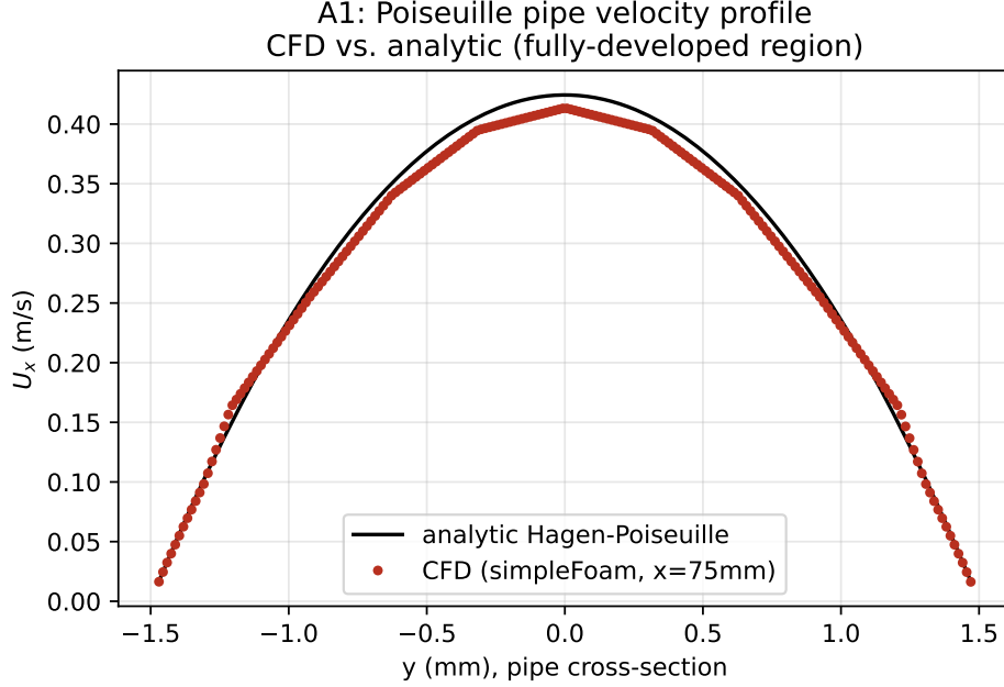
Figure 1: A1: velocity profile at x = 75 \text{ mm} (fully-developed region) against the analytic Hagen–Poiseuille parabola. Peak-velocity agreement is -2.66\% , slightly larger than the -0.75\% pressure-drop error since a point value (peak velocity) is more sensitive to local profile shape than an integral quantity (pressure drop) is.
