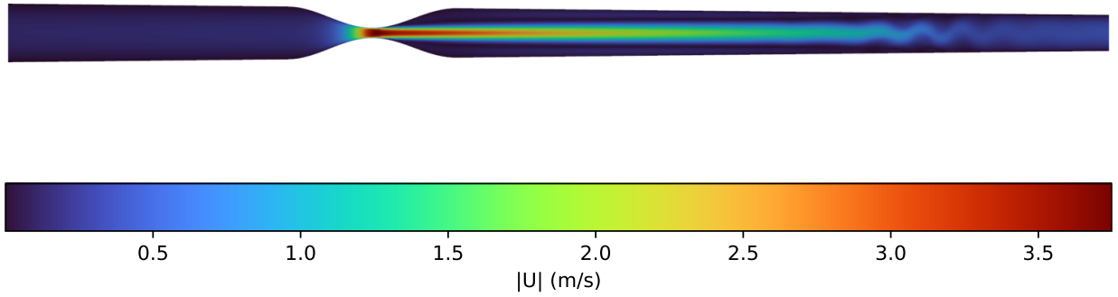
Figure 5: Velocity magnitude, mid-plane slice through the lesion and post-stenotic region ( x=10\text{--}75 mm) at the flagged iteration-2000 state. The jet accelerates sharply through the throat (dark red core, up to 3.75 m/s) and visibly develops a wavy, non-uniform structure downstream — the same post-stenotic region flagged as being at risk of instability.
