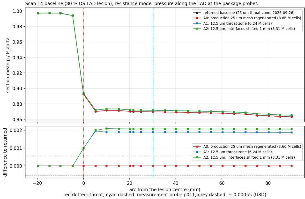
Figure 37: Task A: section-mean p/P_{aorta} at the package probes along the LAD for the returned baseline (25 \mu m), the control A0 (regenerated 25 \mu m), A1 and A2 (12.5 \mu m), and the differences (lower panel; dashed: \pm U_{3D} ). A0 coincides with the returned baseline; A1 and A2 differ from the baseline by at most 1.5 \times 10^{-5} upstream of the lesion and are offset by about +0.002 downstream.
