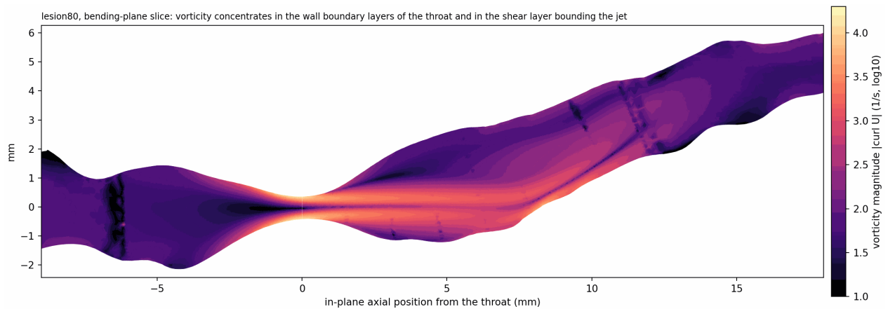
Figure 20: Vorticity magnitude |\nabla \times \mathbf{U}| on the bending-plane slice of lesion80 ( \log_{10} , 1/\text{s} ): the throat wall boundary layers ( \gtrsim 10^4 1/\text{s} ) and the thin shear layer bounding the jet stand out against the low-vorticity recirculation. The thin dark streaks crossing the vessel (at about -6.5 , 3\text{--}4 and 9\text{--}12 mm) are artefacts of the velocity-gradient computation across mesh-refinement interfaces, not flow features.
