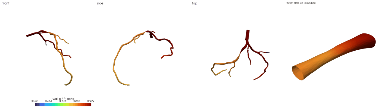
Figure 41: P5 scan 138: wall pressure p/P_{aorta} of the tree in three views and the 6 mm around the throat.
