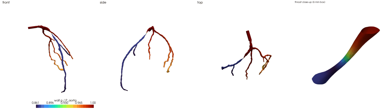
Figure 38: Variant A1: wall pressure p/P_{aorta} of the whole left coronary tree in three views and a close-up of the 6 mm around the throat (same colour scale).
