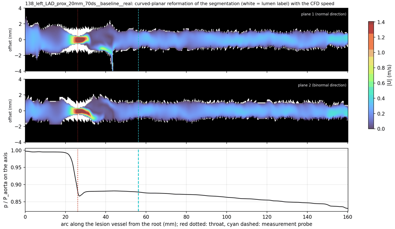
Figure 40: P5 scan 138 (LAD, 20 mm, 70%DS): curved-planar reformation of the unmodified lumen label (white) in two orthogonal planes with the CFD speed |U| in the CFD domain (the synthetic stenosis exists only in the CFD surface), and p/P_{aorta} on the axis (bottom); red dotted: throat, cyan dashed: measurement probe.
