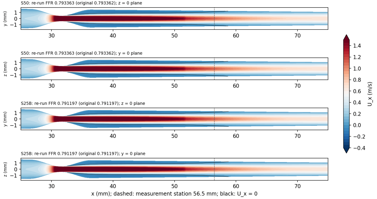
Figure 39: Task B: axial velocity on the two mid-planes of the re-run levels S50 and S25B (throat at 30 mm, U_x = 0 contour in black, dashed: measurement station 56.5 mm). Both jets are axisymmetric and the FFR equals the original value (to 10^{-6} and 3 \times 10^{-8} ). Script code_from_cfd/task_1003/viz/viz_u3d.states.py .
