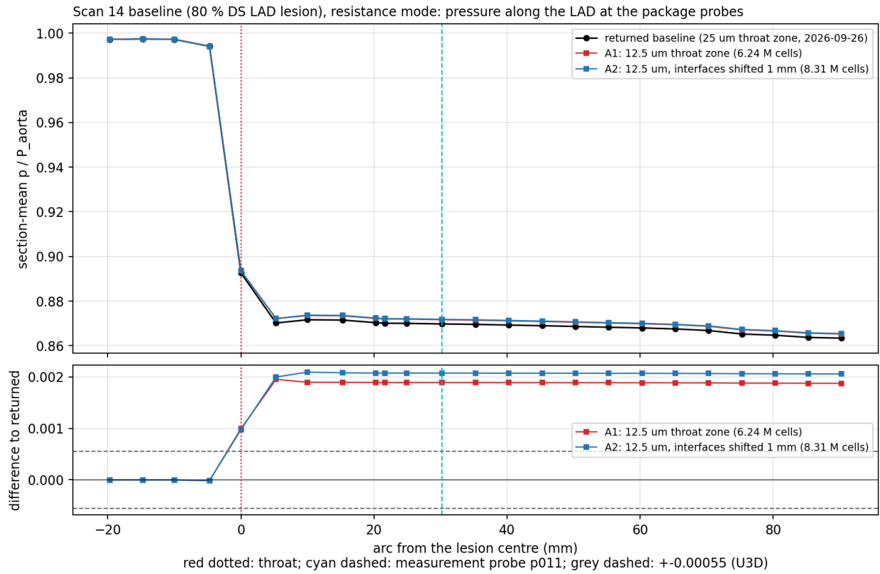
Figure 35: Task A: section-mean p/P_{aorta} at the package probes along the LAD for the returned baseline (25 \mu\text{m} ), A1 and A2 (12.5 \mu\text{m} ), and the differences (lower panel; dashed: \pm U_{3D} ). Identical upstream of the lesion, a constant offset of about +0.002 downstream.
