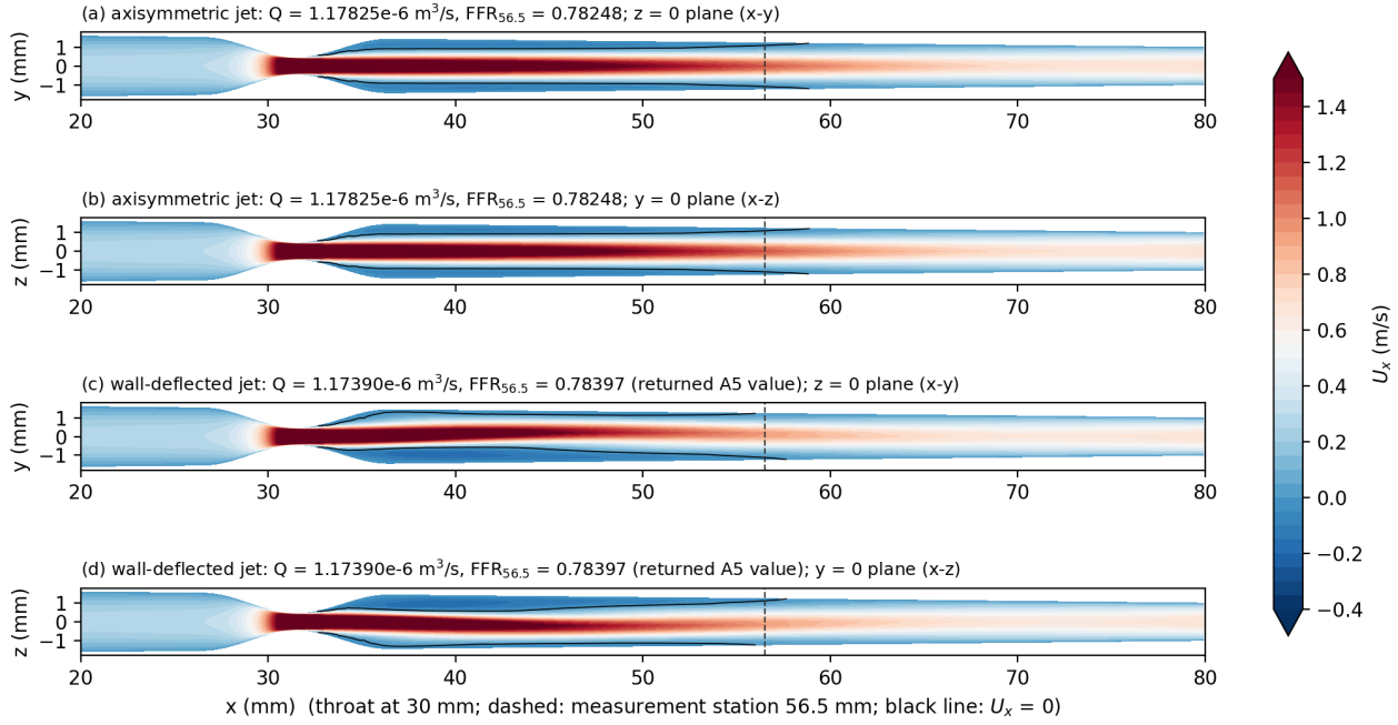
Figure 33: The two steady states of the Stage A sten70 case on the same mesh (the smoke-test mesh of 2026-10-01; state (c,d) obtained by restarting from the archived deflected solution): axial velocity on the two mid-planes, with the U_x = 0 contour (black). (a,b) axisymmetric jet; (c,d) jet deflected towards +y , -z , the state of the returned A5 coarse value. Both are converged (flow band below 10^{-4}\% over 4000 iterations). Script code_from_cfd/task_0926/fig_two_states.py ; jet-offset diagnostic jet_offset.py .
