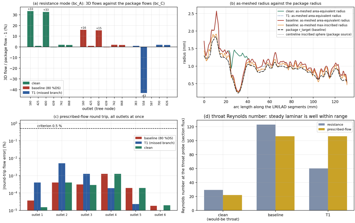
Figure 32: Scan 14, Gate M1: (a) resistance mode, 3D outlet flows against the package flows (bc_C); (b) as-meshed area-equivalent and maximum-inscribed radius along the LM/LAD segments against the package radius; (c) round-trip flow errors of the prescribed-flow mode (all outlets at once); (d) throat Reynolds number from the section flux.
