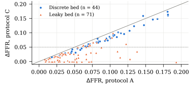
Fig. 4. Change in FFR caused by a missed side branch under fixed boundary conditions (Protocol A) and after tuning to territory flows (Protocol C), paired by instance. The solid line is the identity and the dashed line marks \Delta\text{FFR} = 0.05 .
