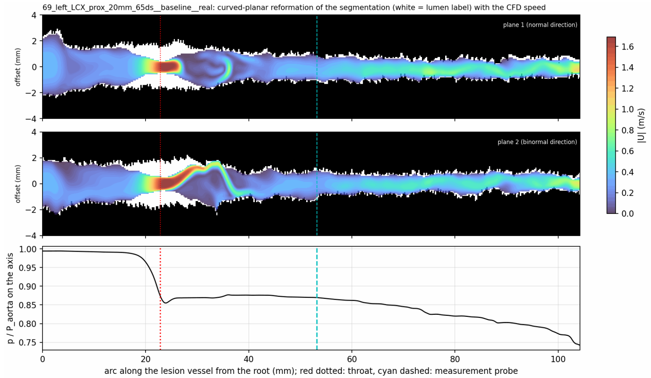
Figure 50: P5 scan 69 (LCx, 20 mm, 65%DS): same layout as for scan 138.
