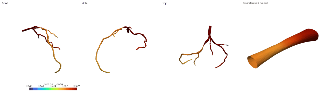
Figure 48: P5 scan 138: wall pressure p/P_{aorta} of the tree in three views and the 6 mm around the throat.
