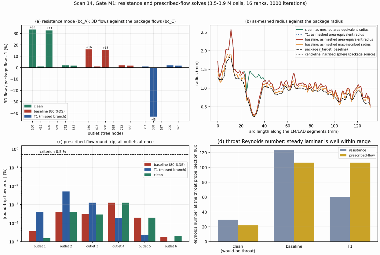
Figure 33: Scan 14, Gate M1: (a) resistance mode, 3D outlet flows against the package flows (bc_C); (b) as-meshed area-equivalent and maximum-inscribed radius along the LM/LAD segments against the package radius; (c) round-trip flow errors of the prescribed-flow mode (all outlets at once); (d) throat Reynolds number from the section flux.
