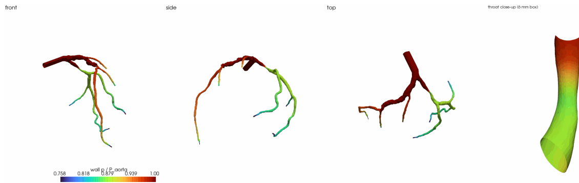
Figure 54: P5 scan 473: wall pressure p/P_{aorta} of the tree in three views and the 6 mm around the throat.
