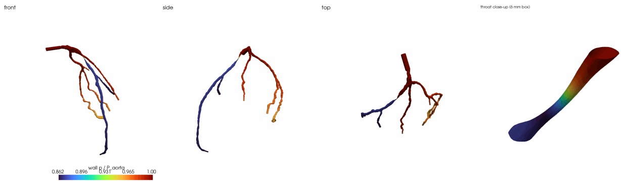
Figure 42: Variant A2 (zone interfaces shifted by 1 mm): wall pressure, same layout and colour scale as Fig. 41.
