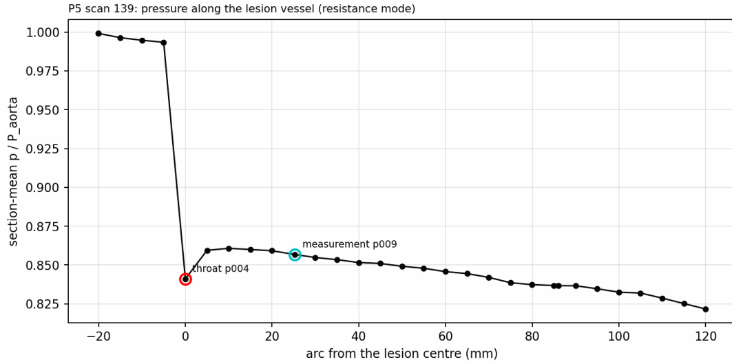
Figure 61: P5 scan 139: section-mean p/P_{aorta} along the lesion vessel at the package probes.
