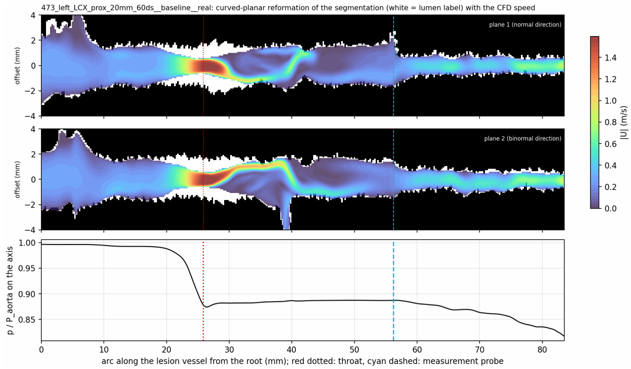
Figure 53: P5 scan 473 (LCx, 20 mm, 60%DS): same layout as for scan 138.
