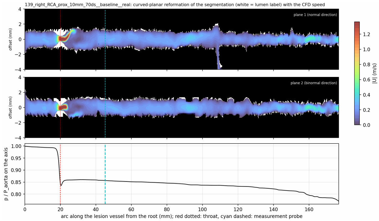
Figure 59: P5 scan 139 (RCA, 10 mm, 70%DS): same layout as for scan 138.
