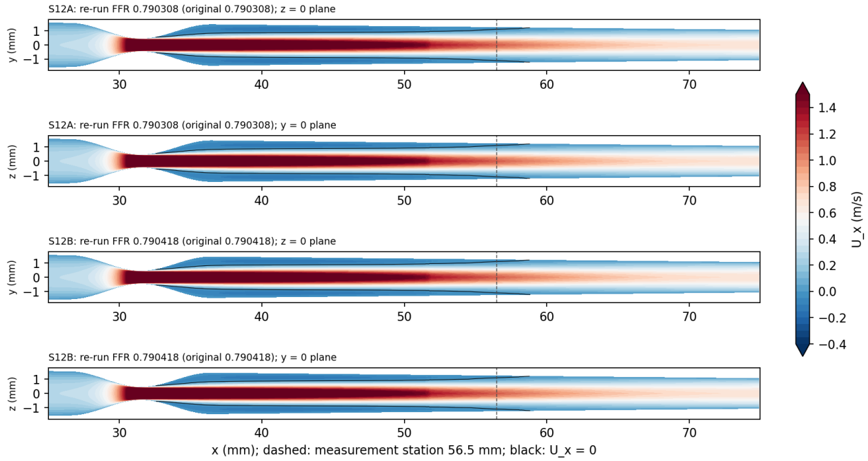
Figure 44: Task B: axial velocity on the two mid-planes of the re-run finest levels S12A (6.7 million cells) and S12B (7.6 million cells), same layout as Fig. 43. Both jets are axisymmetric and the FFR equals the original value ( 3 \times 10^{-7} and 4 \times 10^{-7} ).
