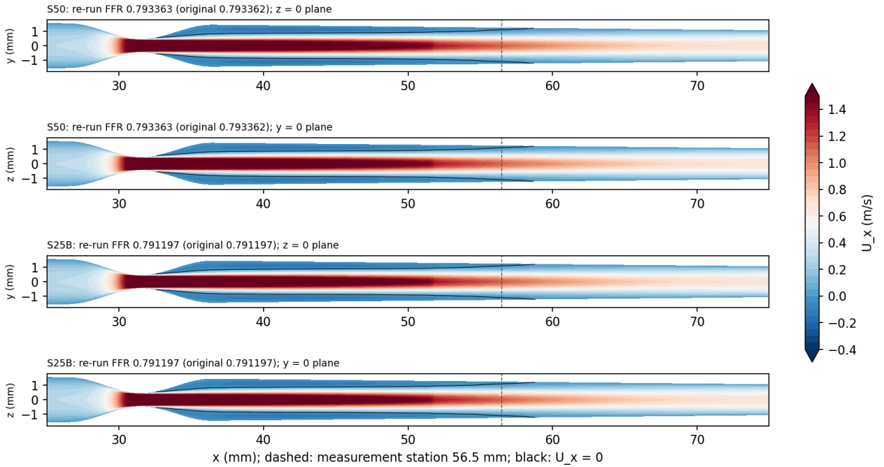
Figure 43: Task B: axial velocity on the two mid-planes of the re-run levels S50 and S25B (throat at 30 mm, U_x = 0 contour in black, dashed: measurement station 56.5 mm). Both jets are axisymmetric and the FFR equals the original value (to 10^{-6} and 3 \times 10^{-8} ). Script code_from_cfd/task_1003/viz/viz_u3d_states.py .
