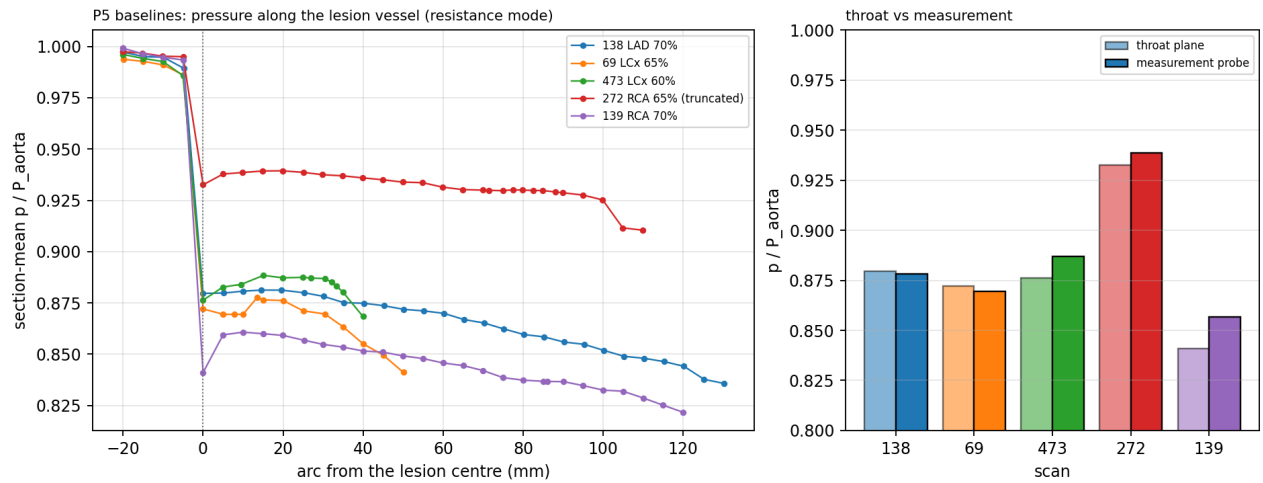
Figure 45: P5 overview. Left: section-mean p/P_{aorta} along the lesion vessel of the five baselines (arc from the lesion centre; resistance mode). Right: p/P_{aorta} at the throat plane and at the measurement probe used. Scan 272 is the truncated-domain solve (outlet out_396 lost in the mesh, 31.5 % of the target flow missing), which is why its pressure drop is small; it is not comparable with the others.
