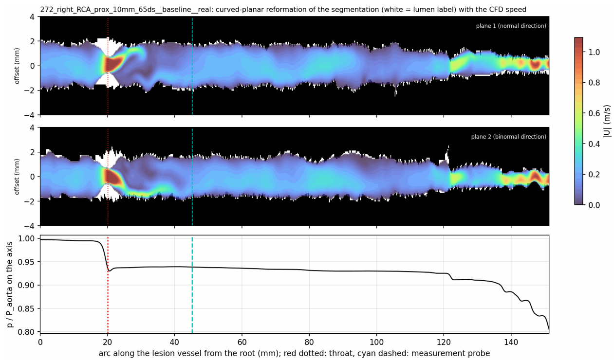
Figure 56: P5 scan 272 (RCA, 10 mm, 65%DS; the outlet out_396 was lost in the mesh and is absent from the solve): same layout as for scan 138.
