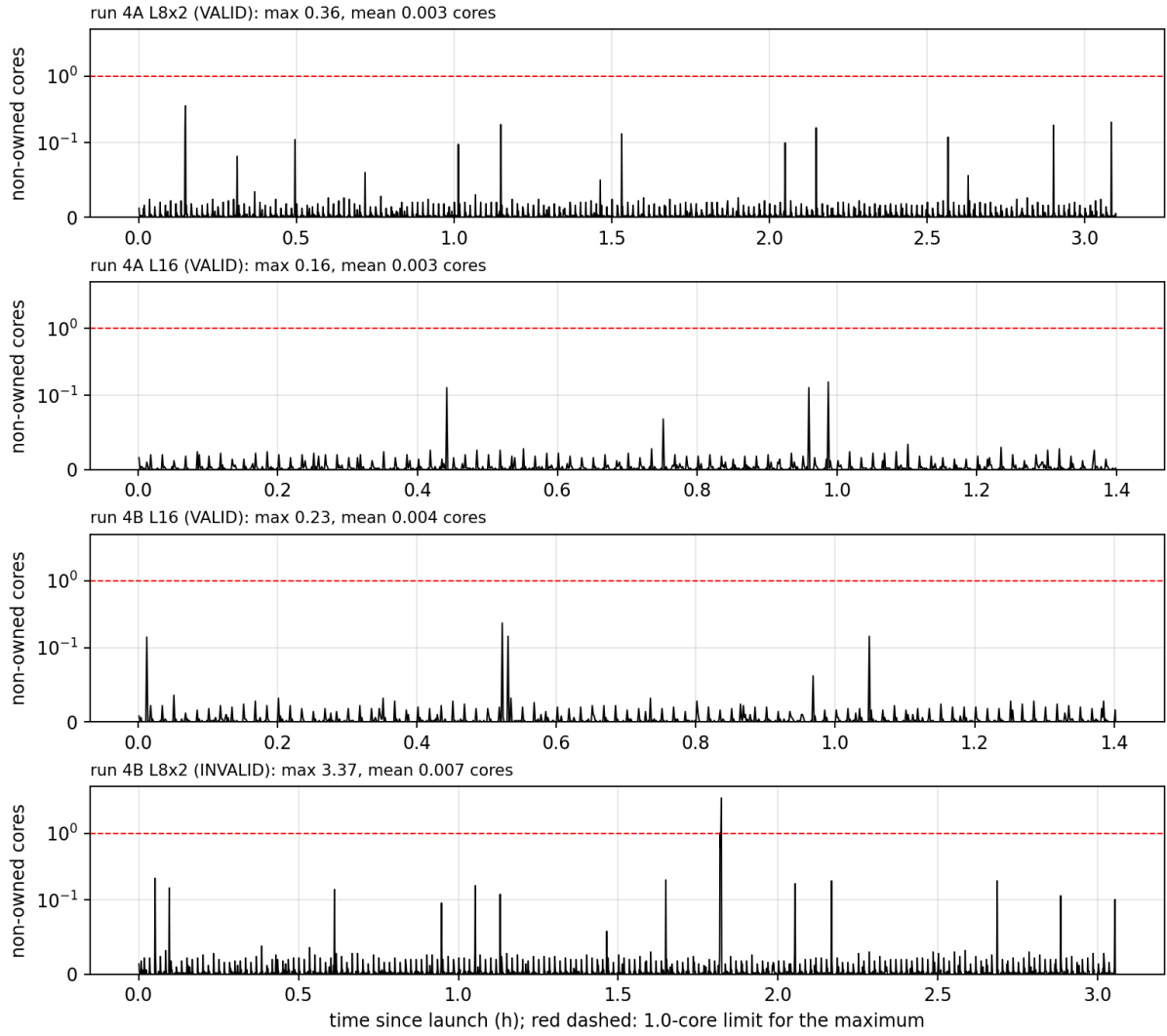
Figure 36: B2 run 4: CPU used by processes not owned by the measurement (cores, symmetric log axis) every 5s during the four layouts. Red dashed: the 1.0-core limit for the maximum. The three VALID layouts stay below 0.4 core; the burst of 3.4 cores in run 4B L8x2 (operating-system update) makes that layout INVALID although the mean is 0.007 core.
