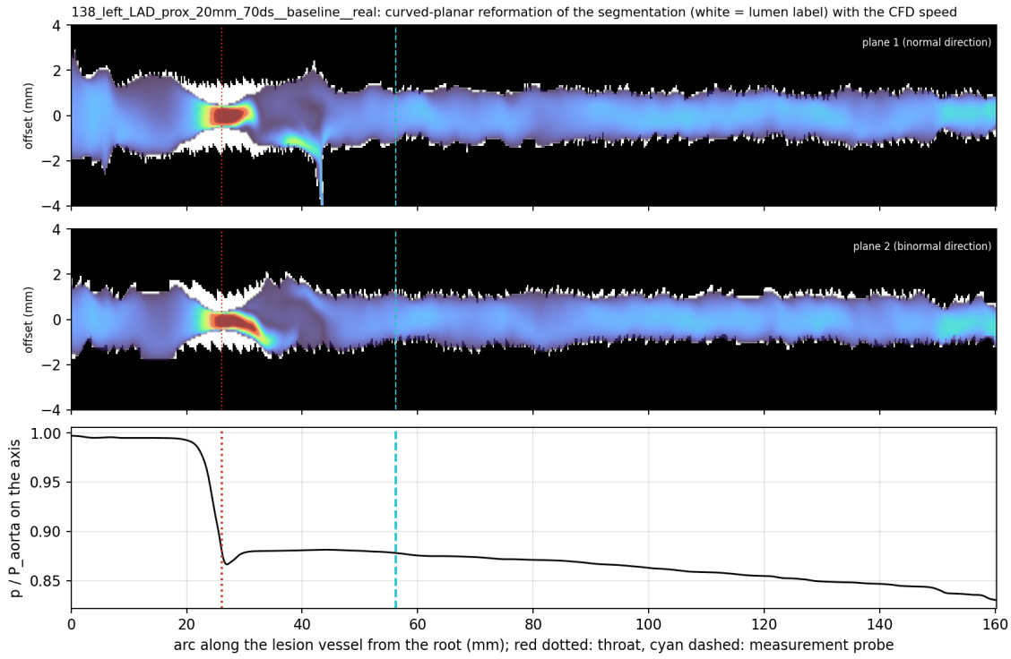
Figure 47: P5 scan 138 (LAD, 20 mm, 70%DS): curved-planar reformation of the unmodified lumen label (white) in two orthogonal planes with the CFD speed |U| in the CFD domain (the synthetic stenosis exists only in the CFD surface), and p/P_{aorta} on the axis (bottom); red dotted: throat, cyan dashed: measurement probe.
