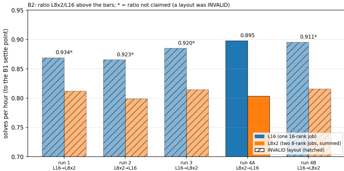
Figure 35: B2: solves per hour to the (proxy) settle point for L16 and L8x2 in the five measurements (runs 1 to 3 and the two pairs of run 4). Hatched: layout INVALID under the strict isolation rule. Above the bars: ratio L8x2/L16; the asterisk marks ratios that are not claimed. Only run 4A has both layouts VALID.
