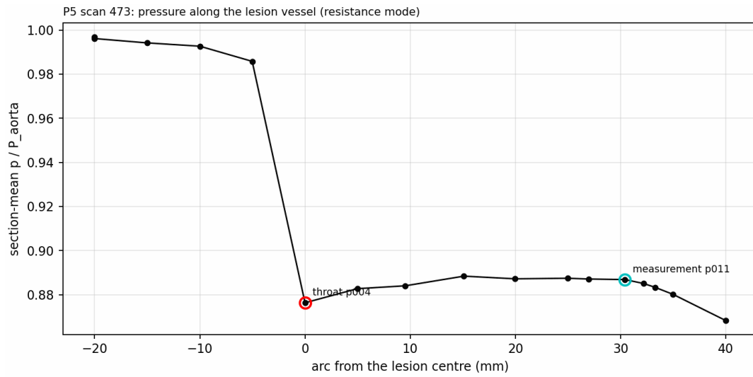
Figure 55: P5 scan 473: section-mean p/P_{aorta} along the lesion vessel at the package probes.
