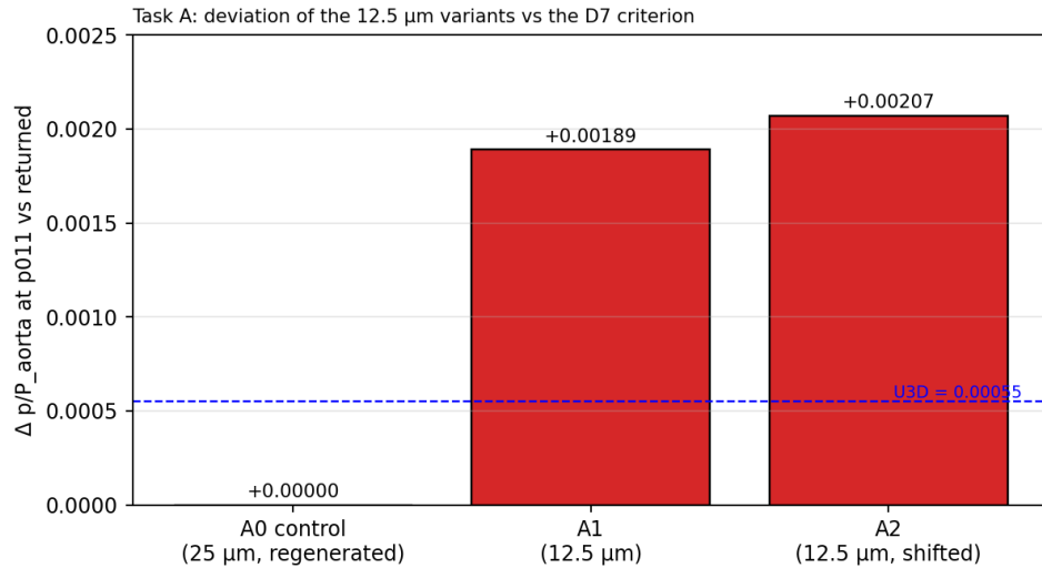
Figure 38: Task A: difference of p/P_{\text{aorta}} at the measurement probe p011 against the returned baseline for the control and the two 12.5 \mu\text{m} variants, against the criterion U_{3D} = 0.00055 (dashed).
