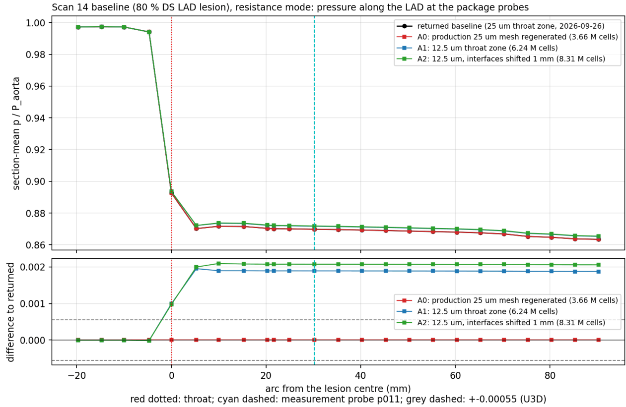
Figure 37: Task A: section-mean p/P_{\text{aorta}} at the package probes along the LAD for the returned baseline (25 \mu\text{m} ), the control A0 (regenerated 25 \mu\text{m} ), A1 and A2 (12.5 \mu\text{m} ), and the differences (lower panel; dashed: \pm U_{3D} ). A0 coincides with the returned baseline; A1 and A2 differ from the baseline by at most 1.5 \times 10^{-5} upstream of the lesion and are offset by about +0.002 downstream.
