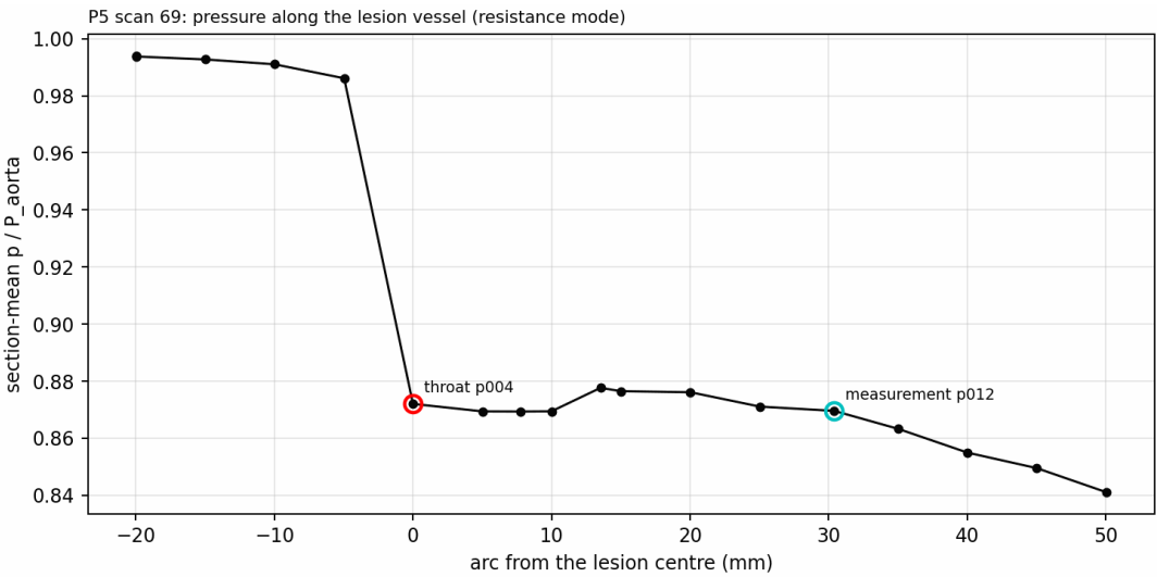
Figure 52: P5 scan 69: section-mean p/P_{aorta} along the lesion vessel at the package probes.
