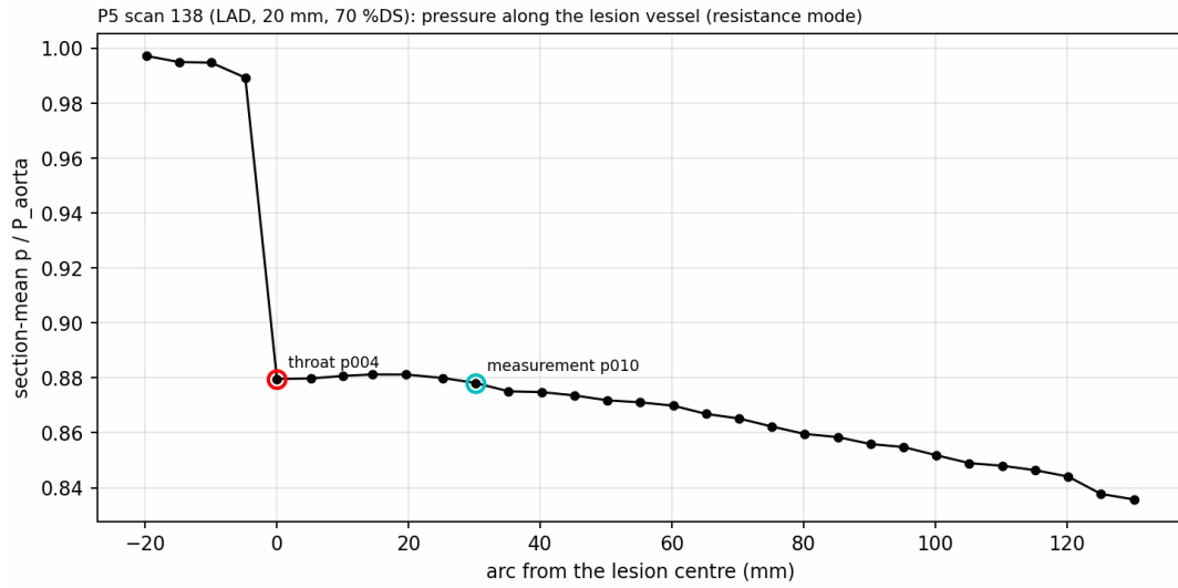
Figure 49: P5 scan 138: section-mean p/P_{aorta} at the package probes along the lesion vessel (resistance mode), with the throat and measurement probes marked.
