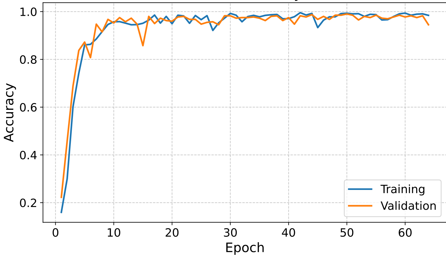
Model Accuracy
