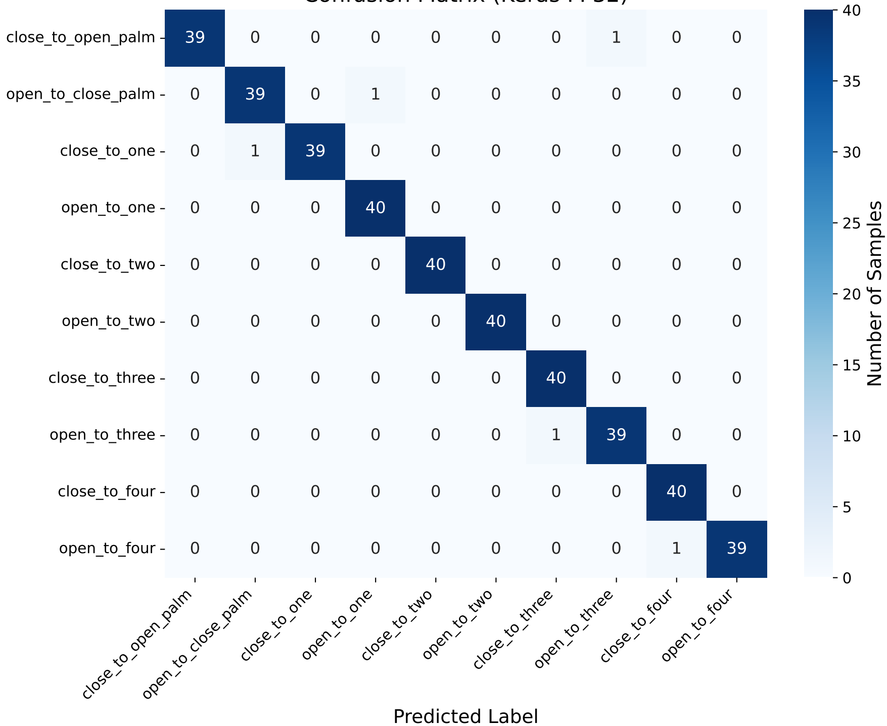
Confusion Matrix (Keras FP32)
