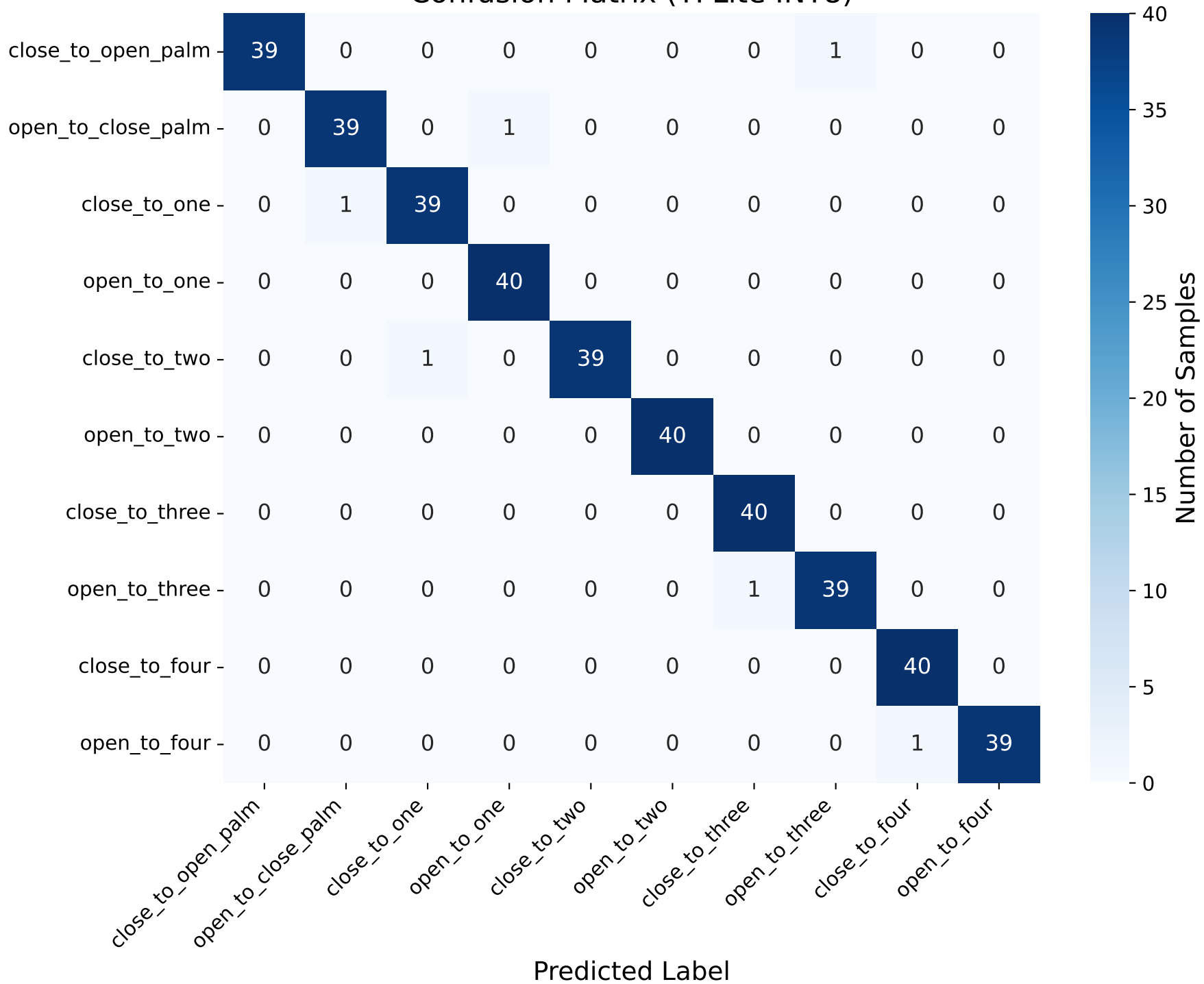
Confusion Matrix (TFLite INT8)
