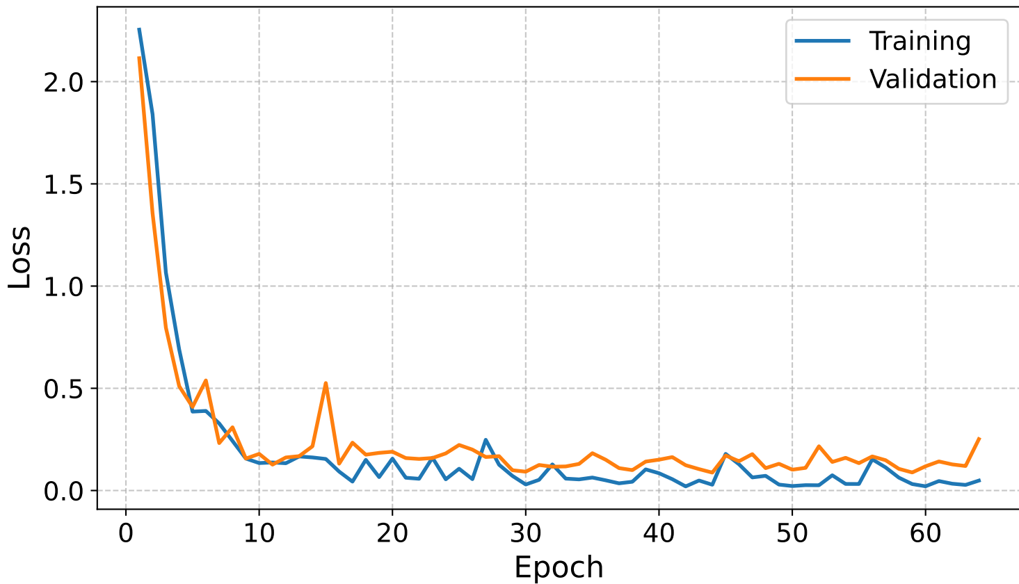
Model Loss
