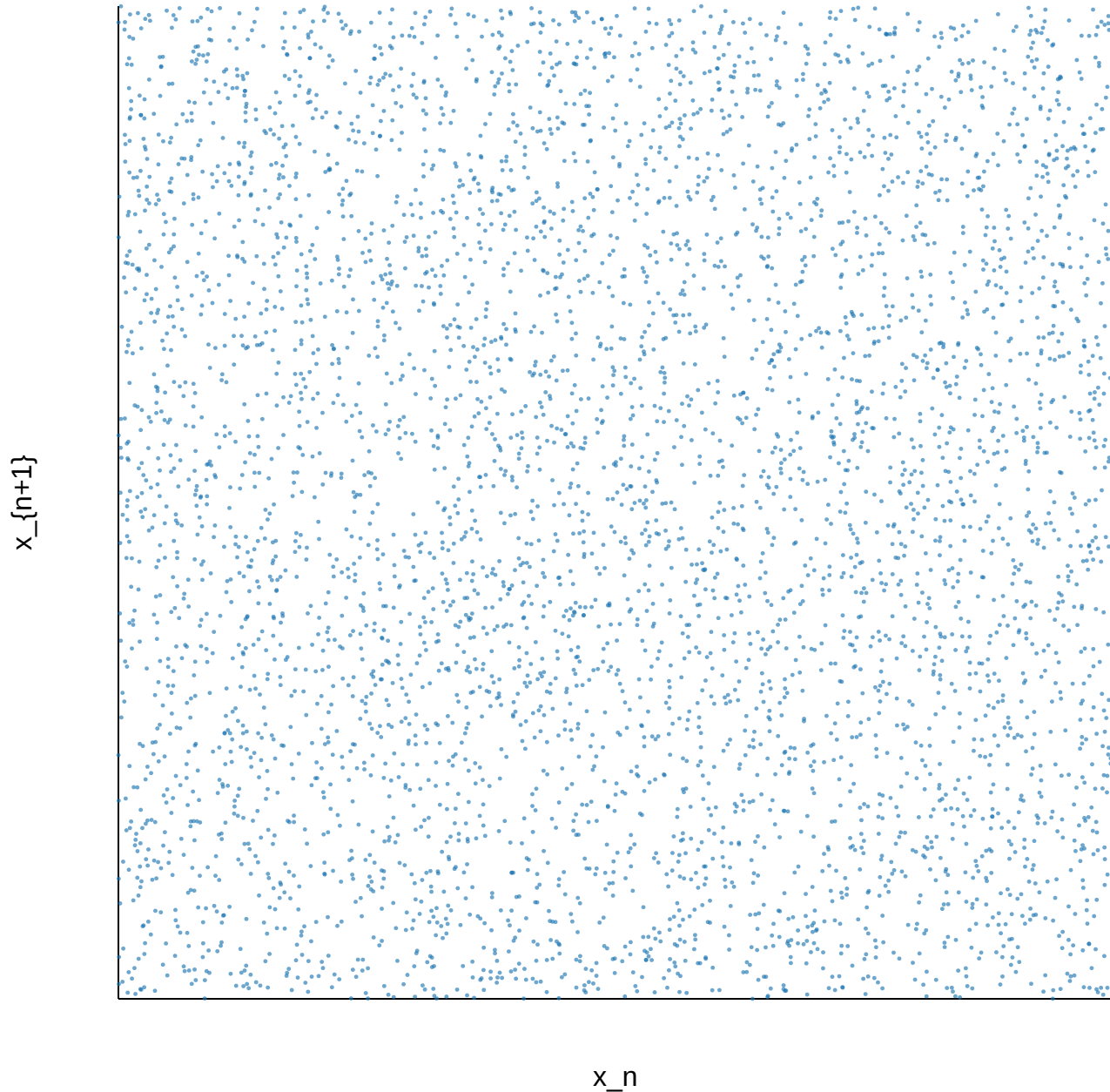
LCG with one broken Hull-Dobell condition successive values
