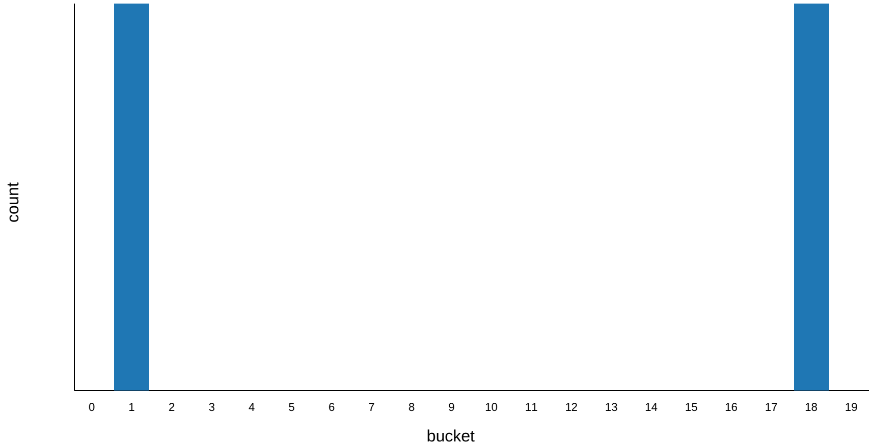
Bad Lehmer large range histogram
