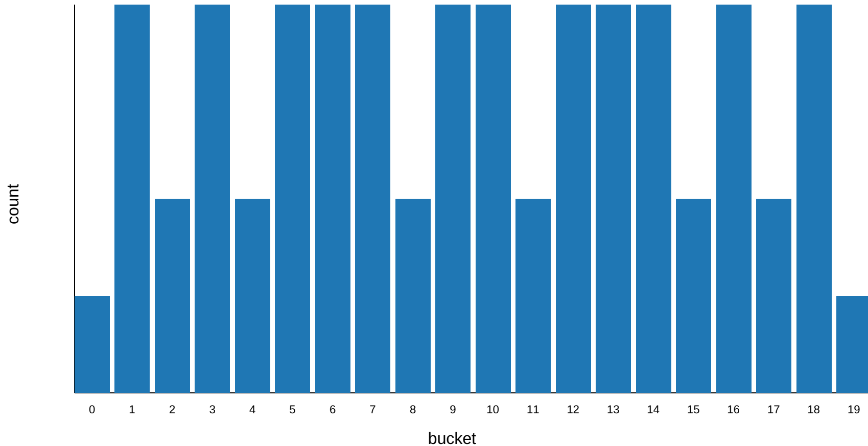
Lehmer with non-primitive multiplier histogram
