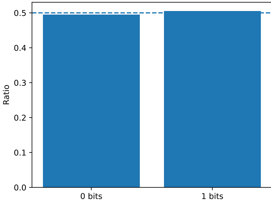
Bad additive LFG short lags 1-2 bit ratio
