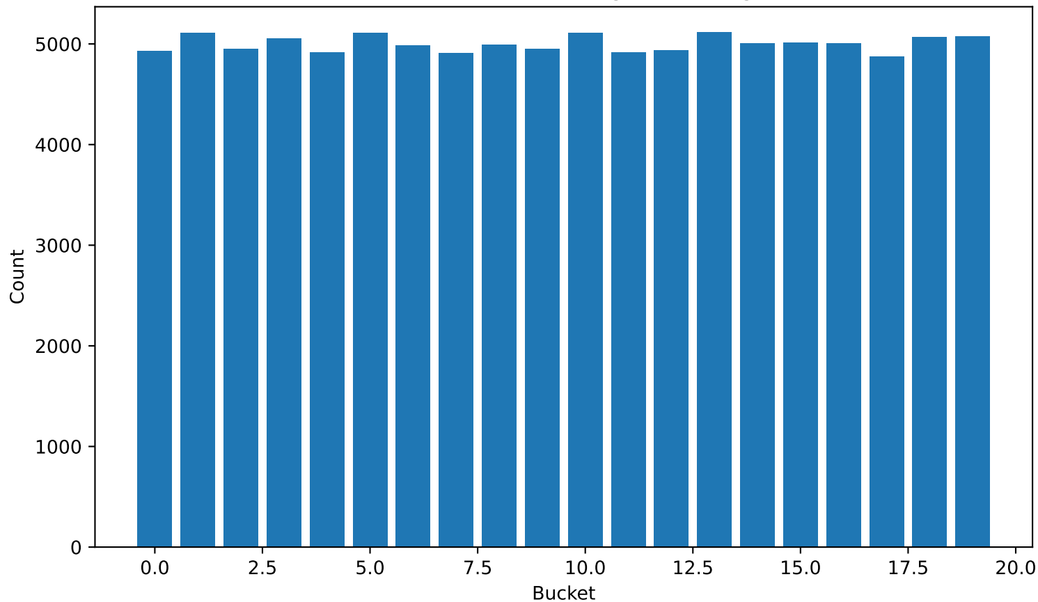
Bad additive LFG short lags 1-2 histogram
