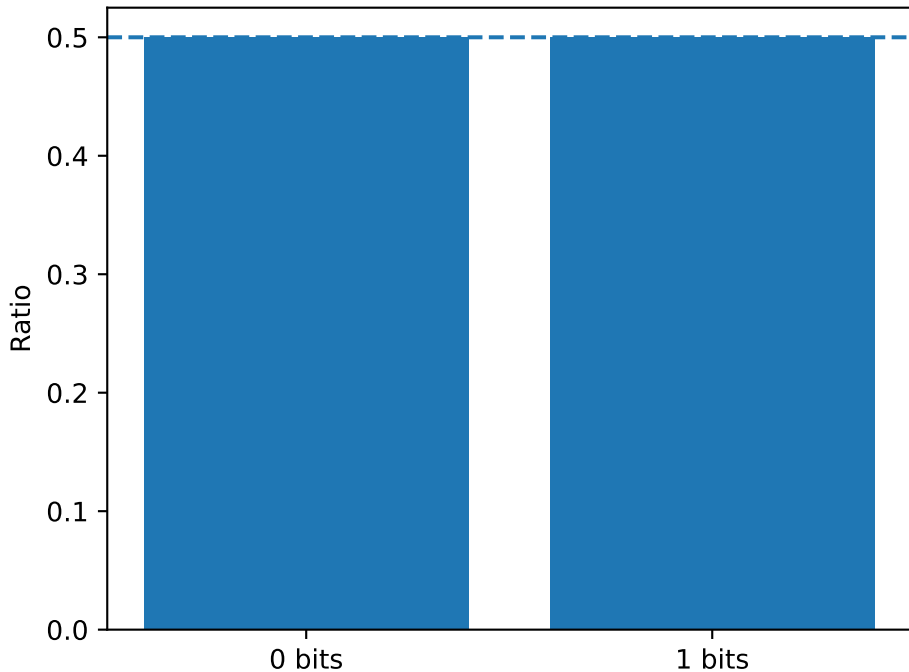
Bad 32-bit LFSR single tap bit ratio
