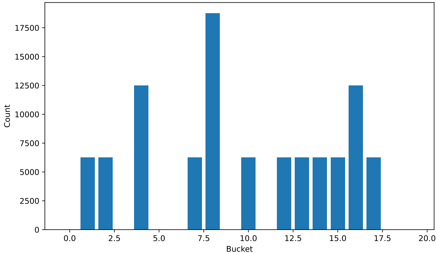
Bad 32-bit LFSR single tap histogram
