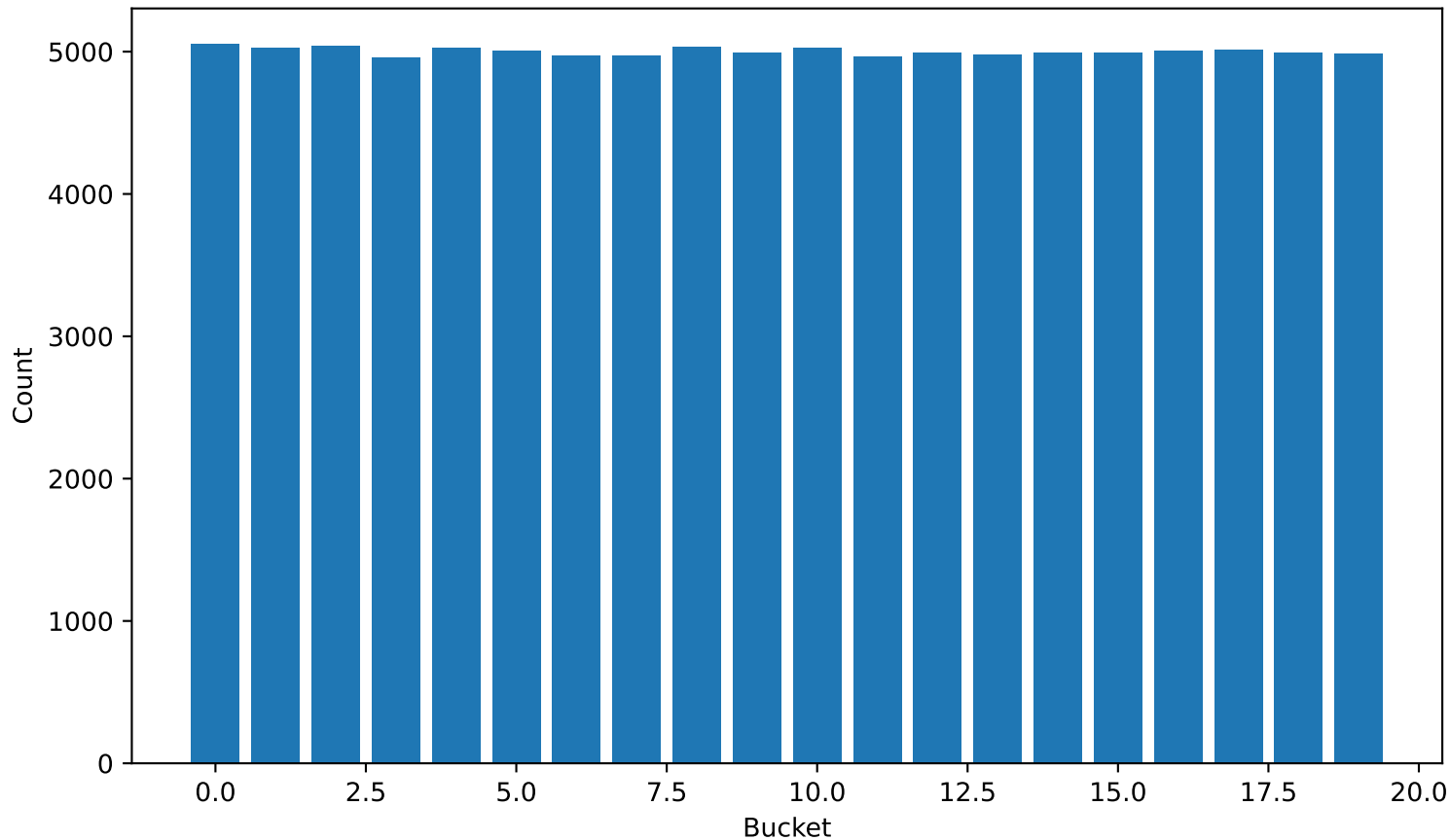
Good 16-bit LFSR histogram
