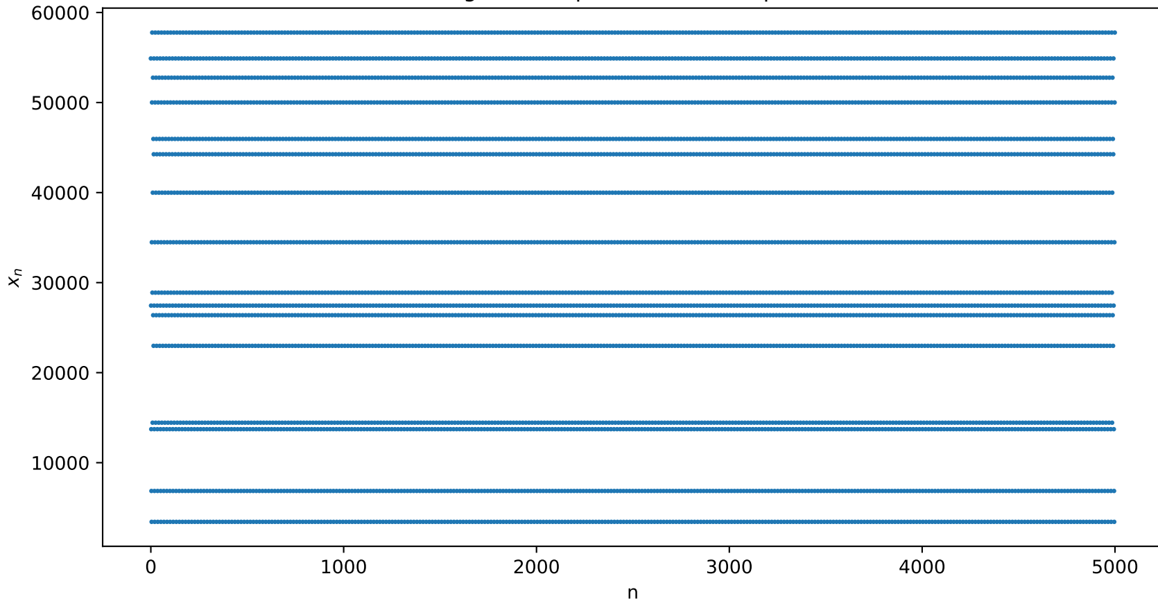
Single bad tap 16-bit LFSR sequence
