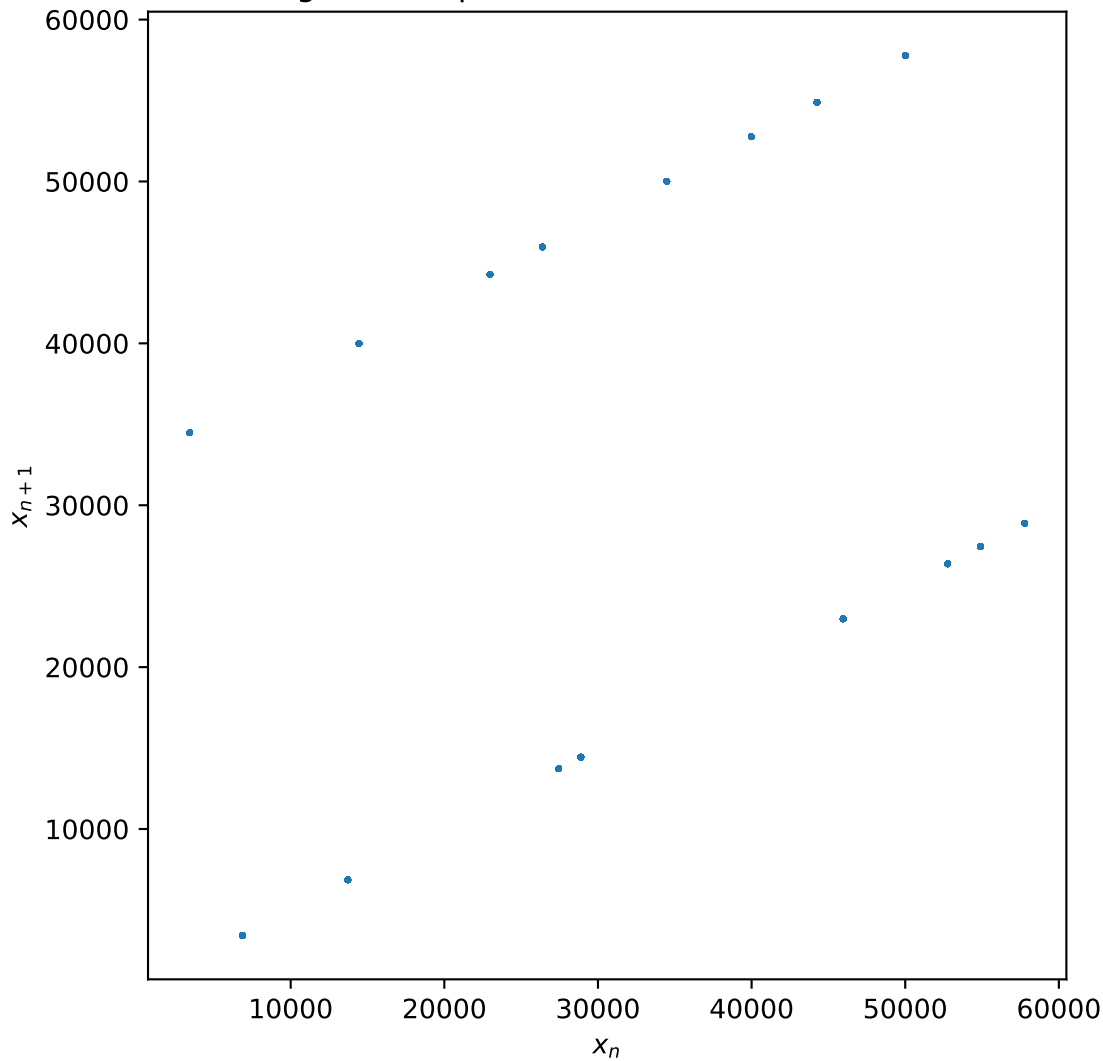
Single bad tap 16-bit LFSR successive values
