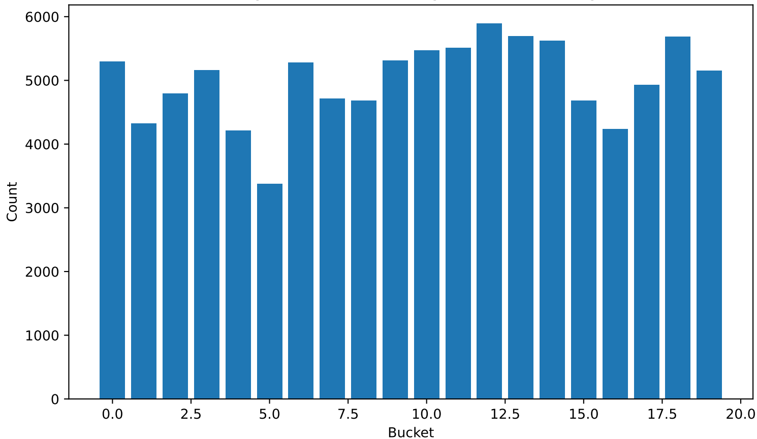
MT-like generator with missing twist matrix histogram
