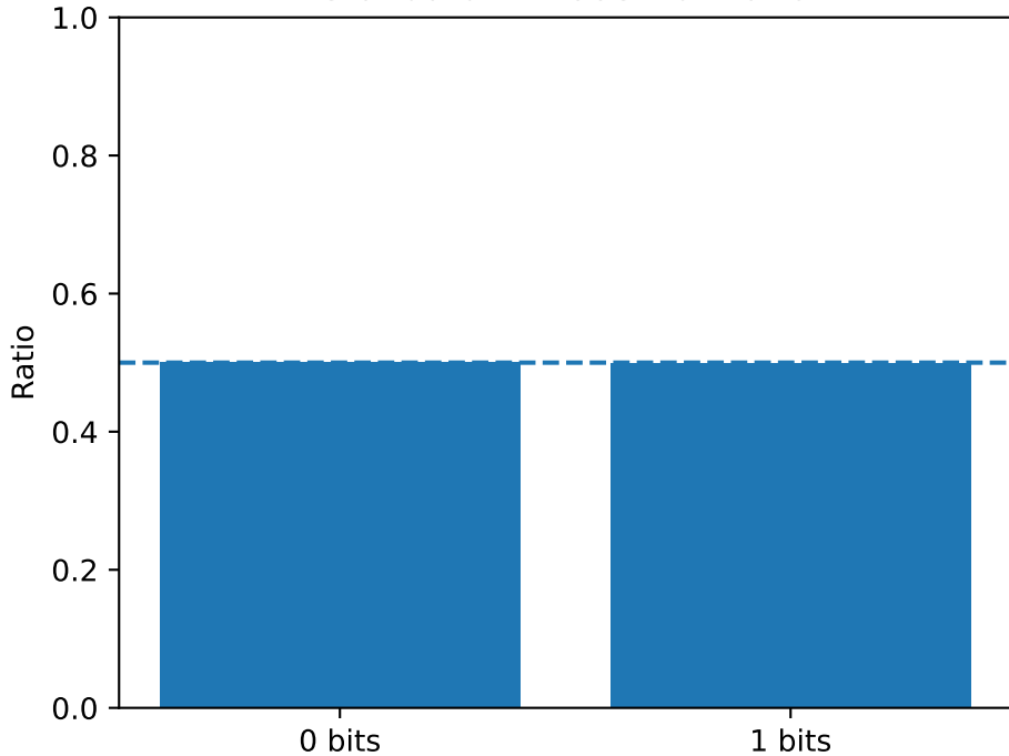
Standard MT19937 bit ratio
