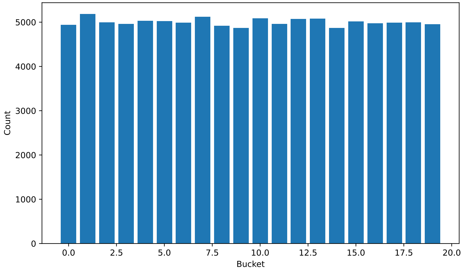
Standard MT19937 histogram
