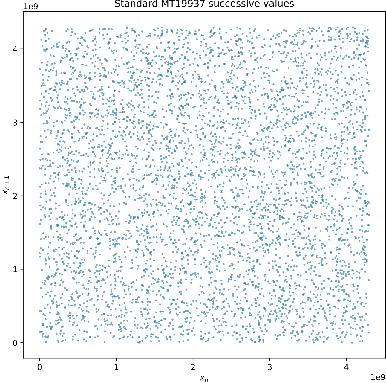
Standard MT19937 successive values
