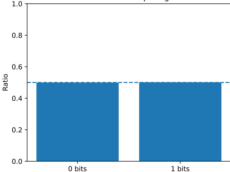
MT19937 without tempering bit ratio
