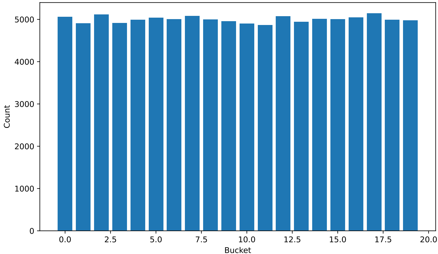
MT19937 without tempering histogram
