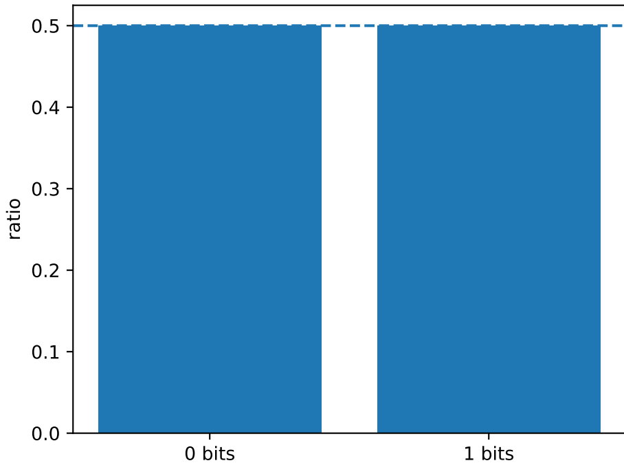
PCG32 even increment bit ratio
