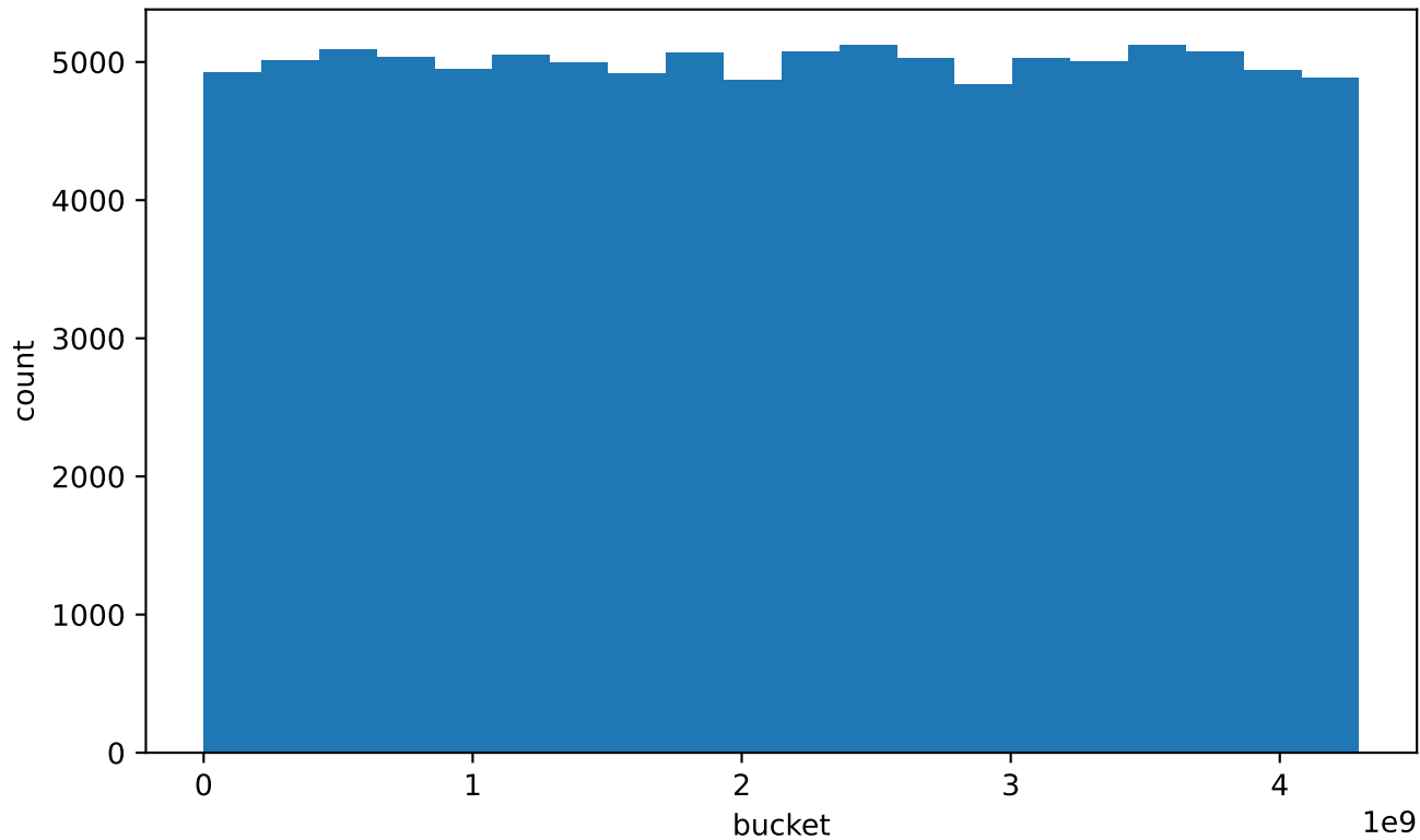
PCG32 even increment histogram
