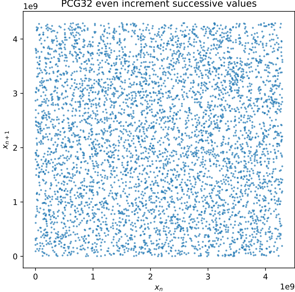
PCG32 even increment successive values
