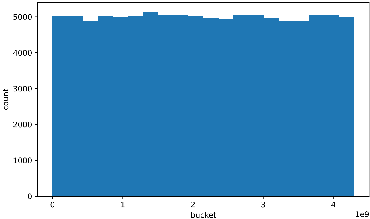
PCG32 good stream histogram
