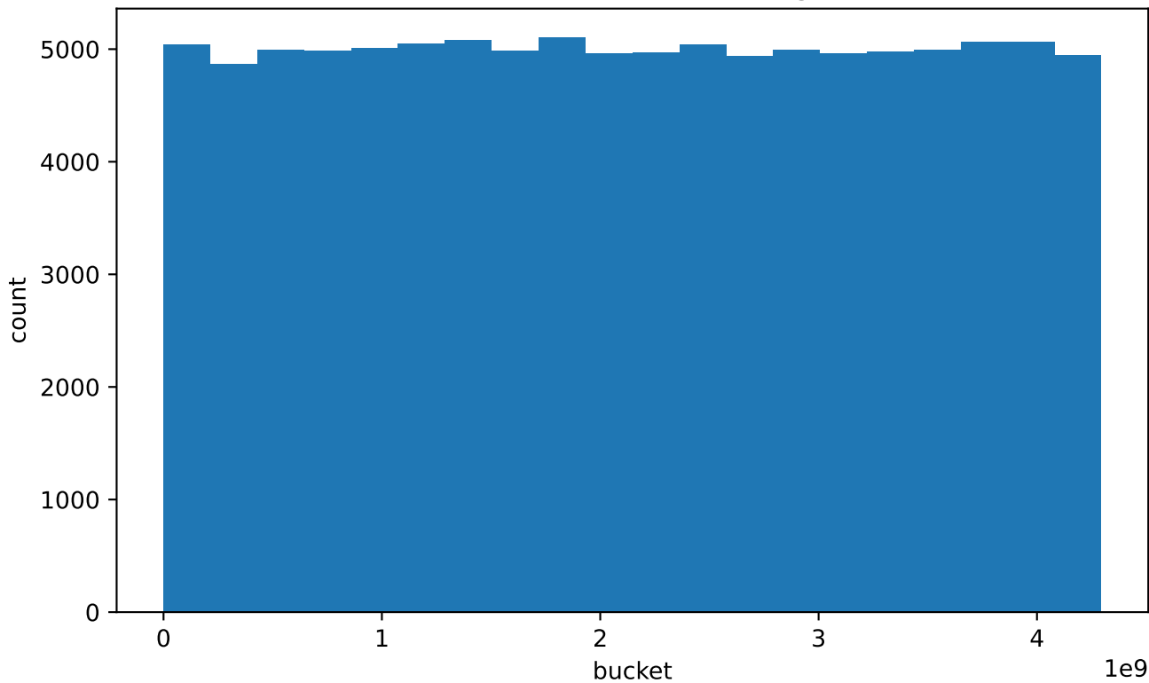
PCG32 zero increment histogram
